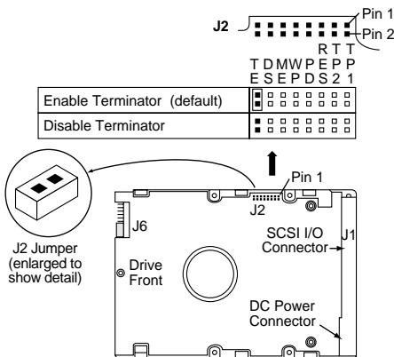
Figure 13. Terminating the drive (“W” model shown)
