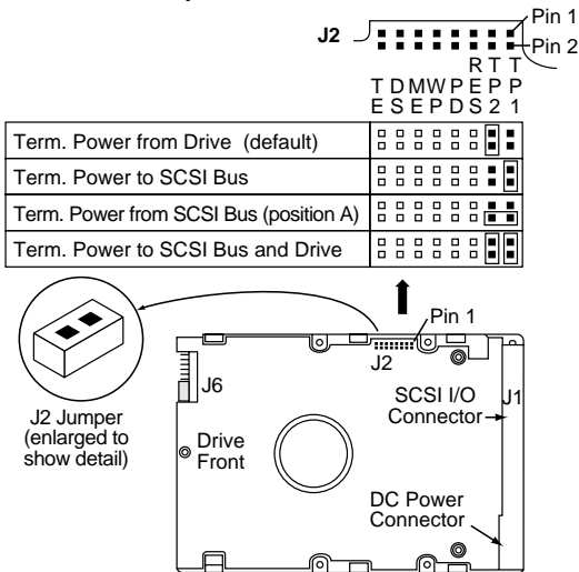
Figure 9. Setting terminator power jumpers
