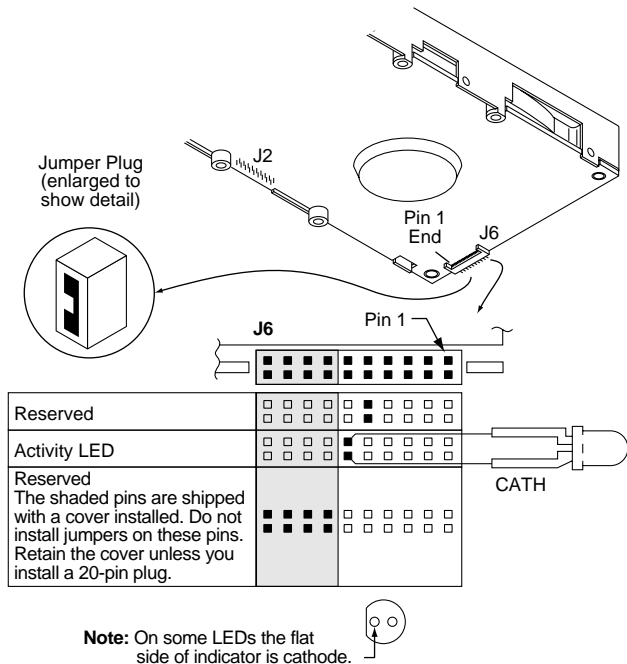
Figure 17. Drive Active LED indicator connections
