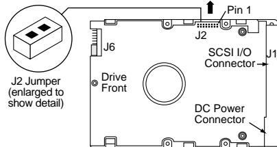
Figure 10. Additional jumper options
