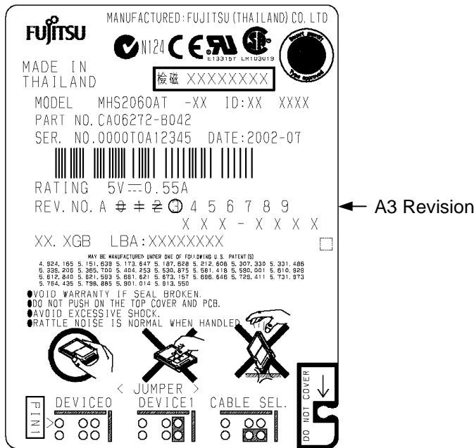
Figure 1.2 Display of disk drive revision number
