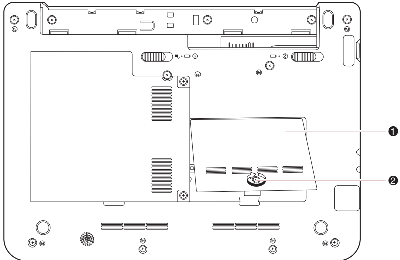
Figure 8-3 Seating the memory module cover
