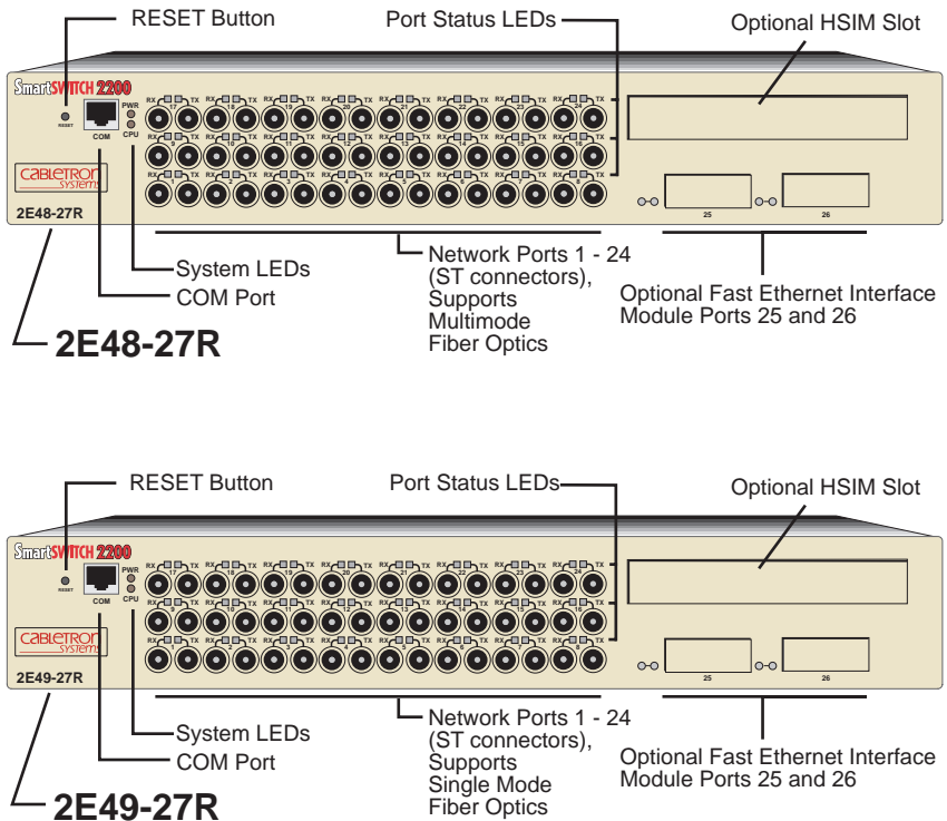
Figure 1-1 The 2E48-27R and 2E49-27R
