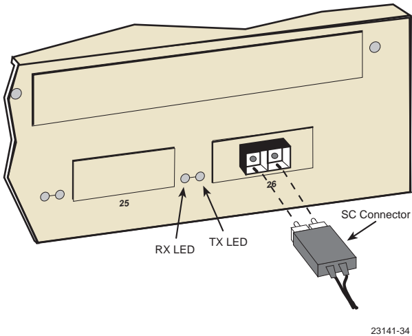
Figure 3-9 FE-100FX or FE-100F3 Port Connection
