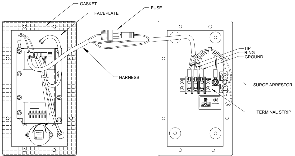
Figure 3 - Installation SCR-11
