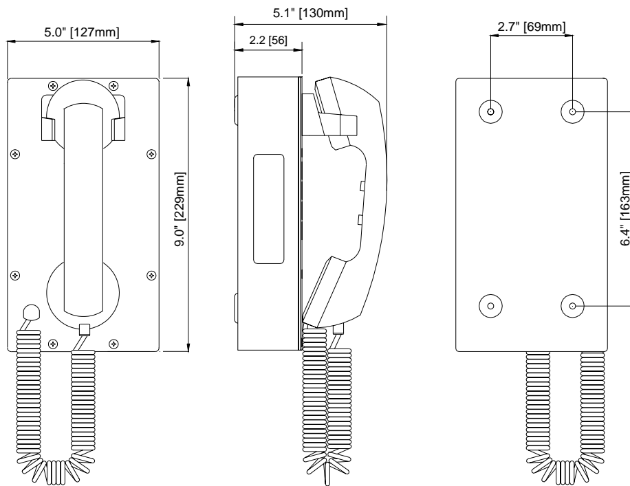
Figure 2 - Overall Dimensions
