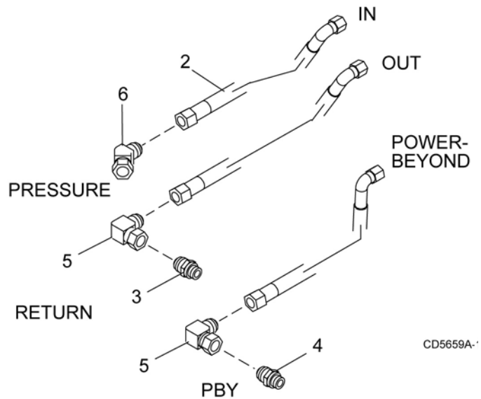
Figure 18. Hydraulic Fitting and Hose Installation
