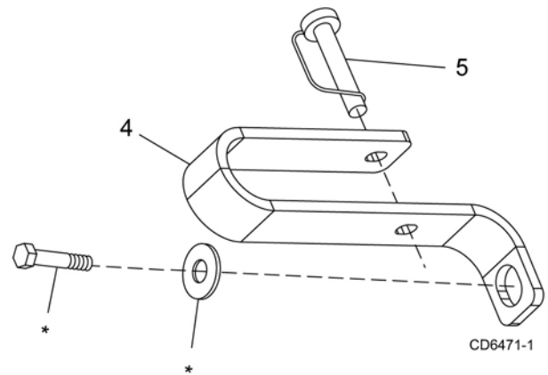
Figure 41. Hose Hanger Installation
