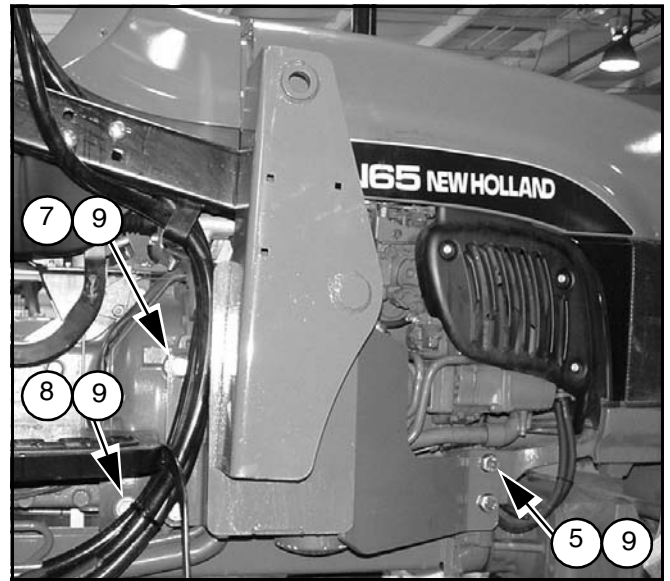
Figure 1. Right Rear Mount Installed
