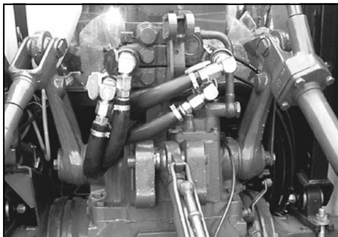
Figure 6. Connections to Tractor Hydraulic Couplers (Typical)
