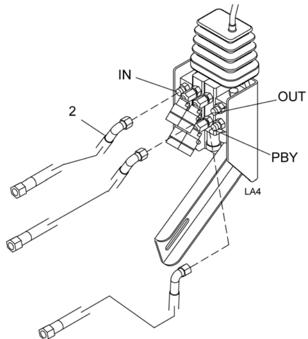
Figure 16. Control Valve Hose Connections
