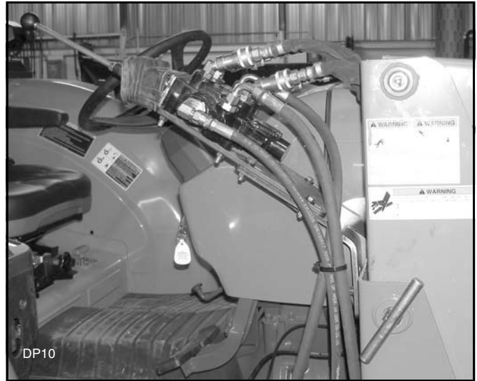
Figure 43. Control Valve Installed (Typical)
