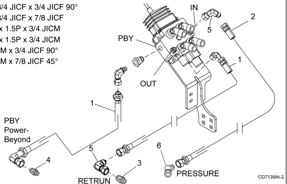
Figure 47. Hydraulic Fittings and Hose Installation
