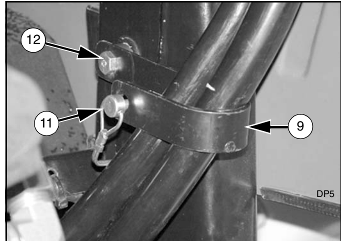
Figure 49. Hose Hanger Installed
