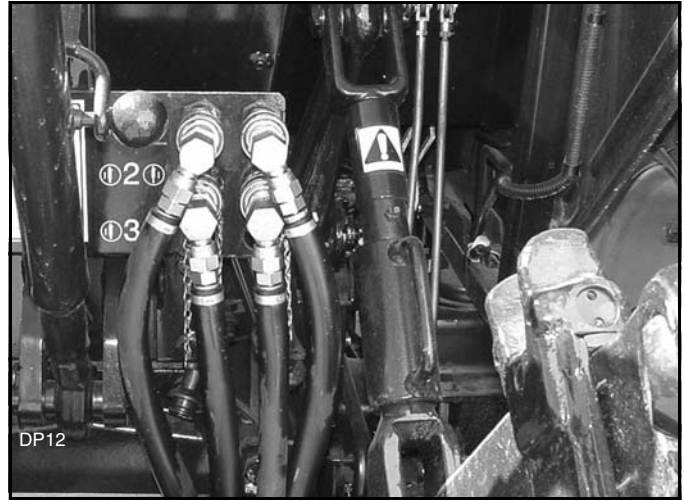
Figure 38. Tractor Rear Hydraulic Couplers (Typical)
