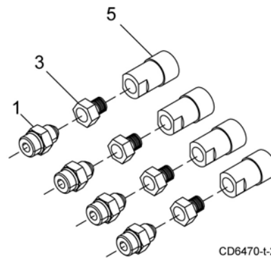
Figure 26. Hydraulic Fitting Installation
