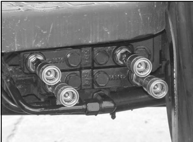
Figure 25. Hydraulic Fittings Installed
