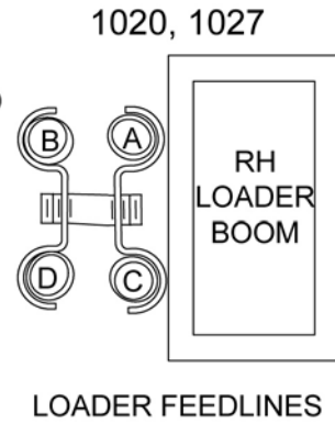
Figure 7. Loader Feedline Connection
