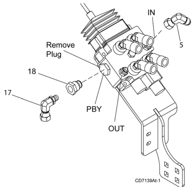
Figure 44. Cable Control Valve Fitting Installation
