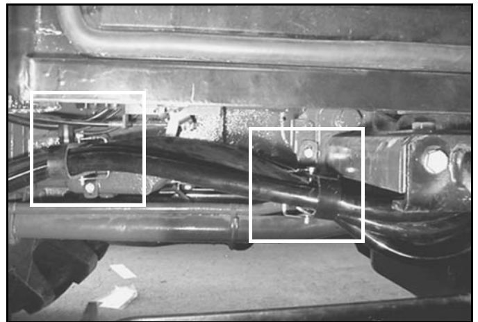
Figure 10. Hose Hangers Installed
