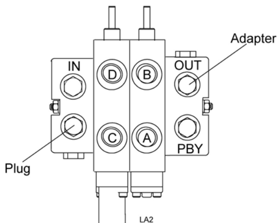
Figure 14. Correct Control Valve Arrangement
