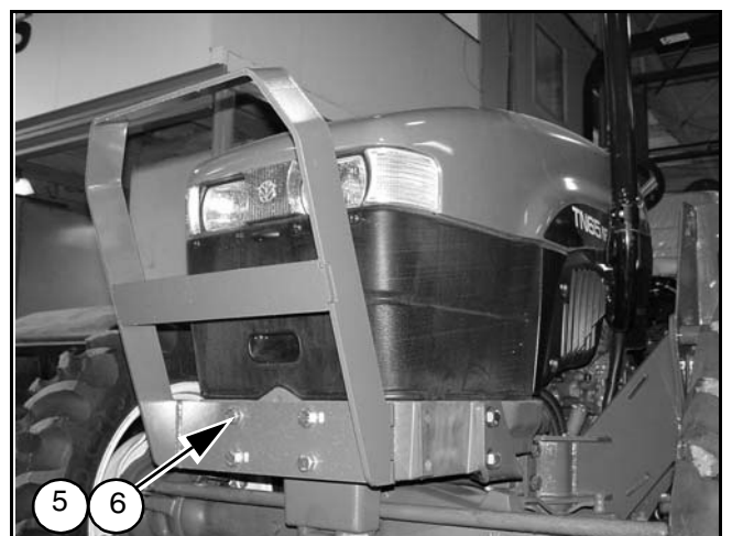
Figure 3. Grill Guard Installed
