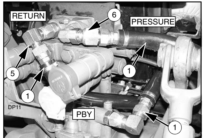
Figure 46. Hydraulic Fittings and Hose Connections
