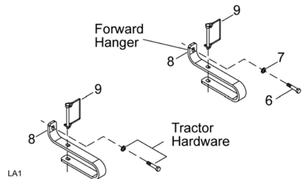
Figure 11. Hose Hanger Installation
