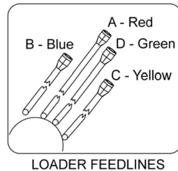
Figure 50. LU126 & LU132 Control Valve and Loader Feedline Hose Connections
