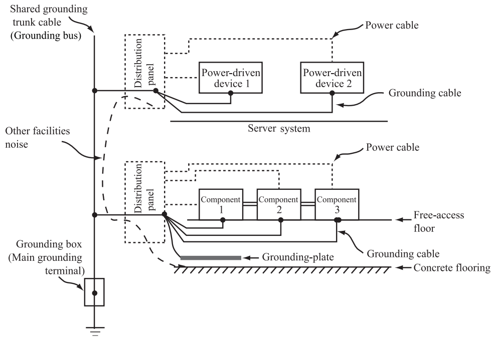
Figure 6.6 Grounding-plate method
