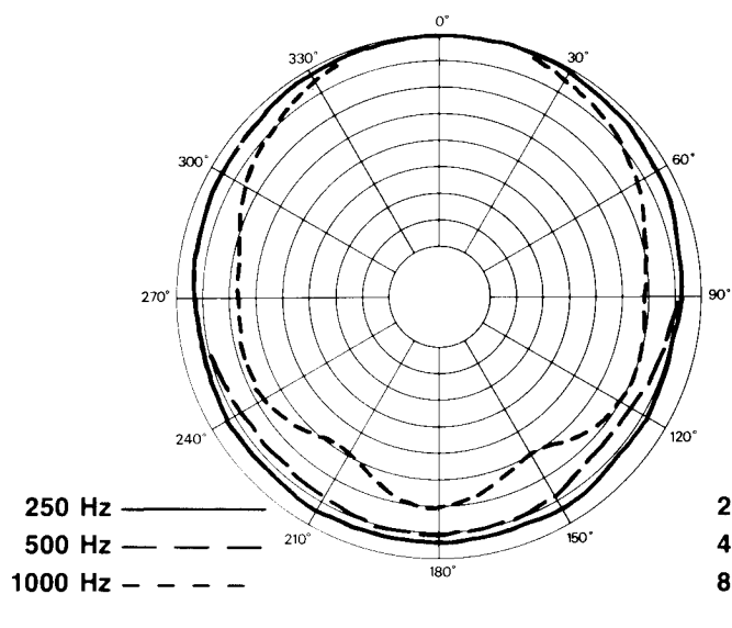
FIGURE 3A — PRO-8A Polar Response in 0.25 ft 3 Sealed Box 4V RMS of 1/3-Octave-Band-Limited Noise in Anechoic Environment, 10 Feet on Axis (5 dB per division)
