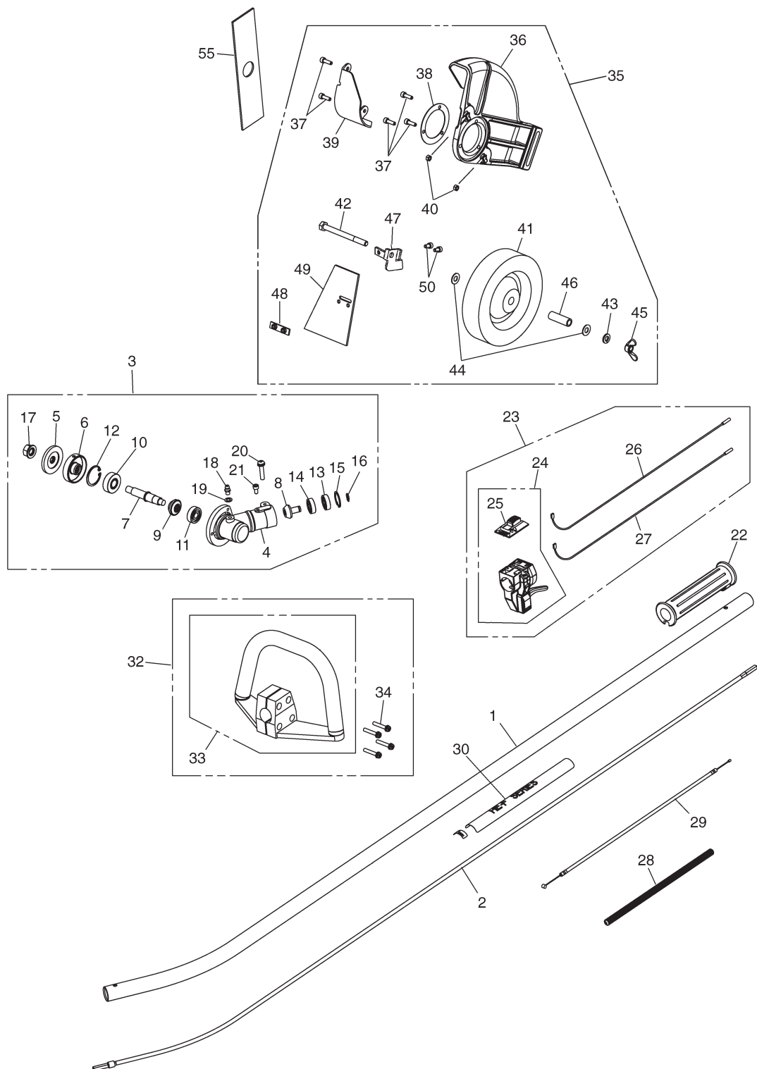
Fig.1 DRIVE UNIT HE250F (S/N 70200101 and up)
