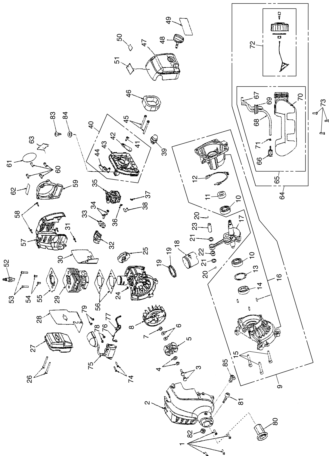
Fig.2 ENGINE UNIT HE250F (S/N 70200101 and up)
