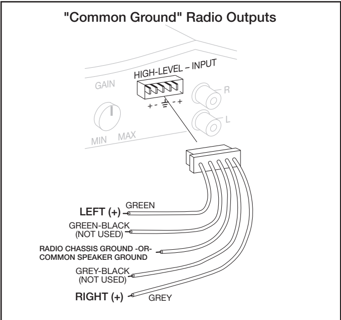
High Level (Speaker Input) Wiring
