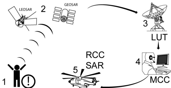
COSPAS-SARSAT System concept
