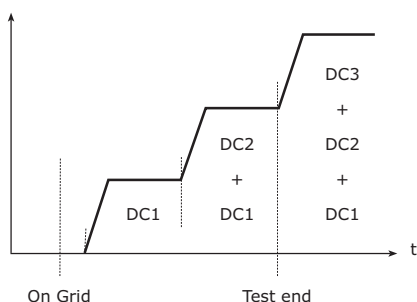
Illustration 2.1: PV-konfigurationstest
