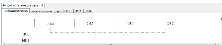
Figure 13.1: Architectural overview
