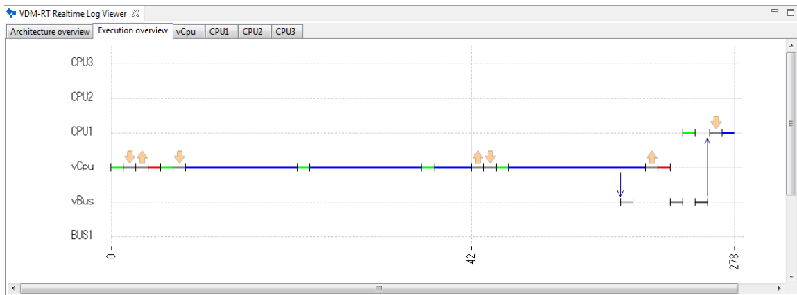
Figure 13.2: Execution overview
