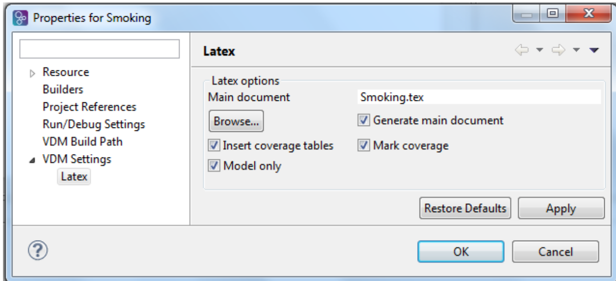
Figure 4.4: Overture Project Settings for \LaTeX
