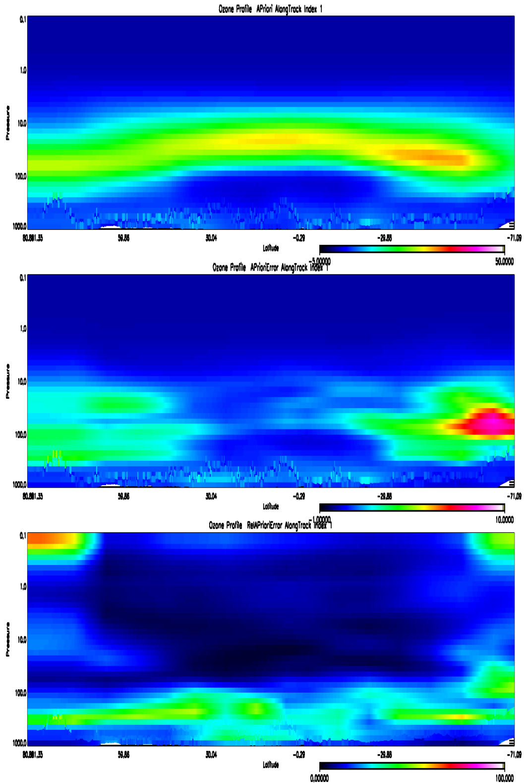
Figure 10: A priori ozone profile (top), its error (center) and relative error (bottom). The example refers to orbit 4679 (A) of GOME-2 on Metop-A.
