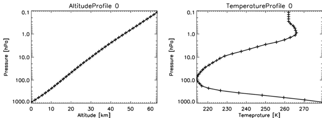
Figure 6: Relation between pressure and altitude and the temperature profile for an example retrieval.
