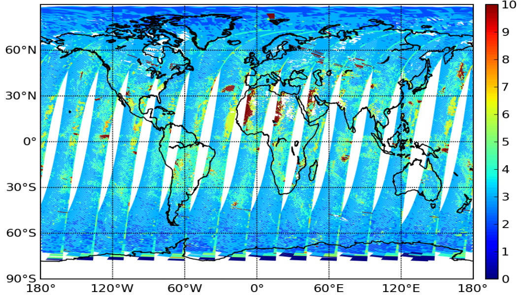
Figure 13: Number of iterations for each retrieval from GOME-2 on Metop-B on March 29 th 2013. Brown pixels indicate non-converged profiles.
