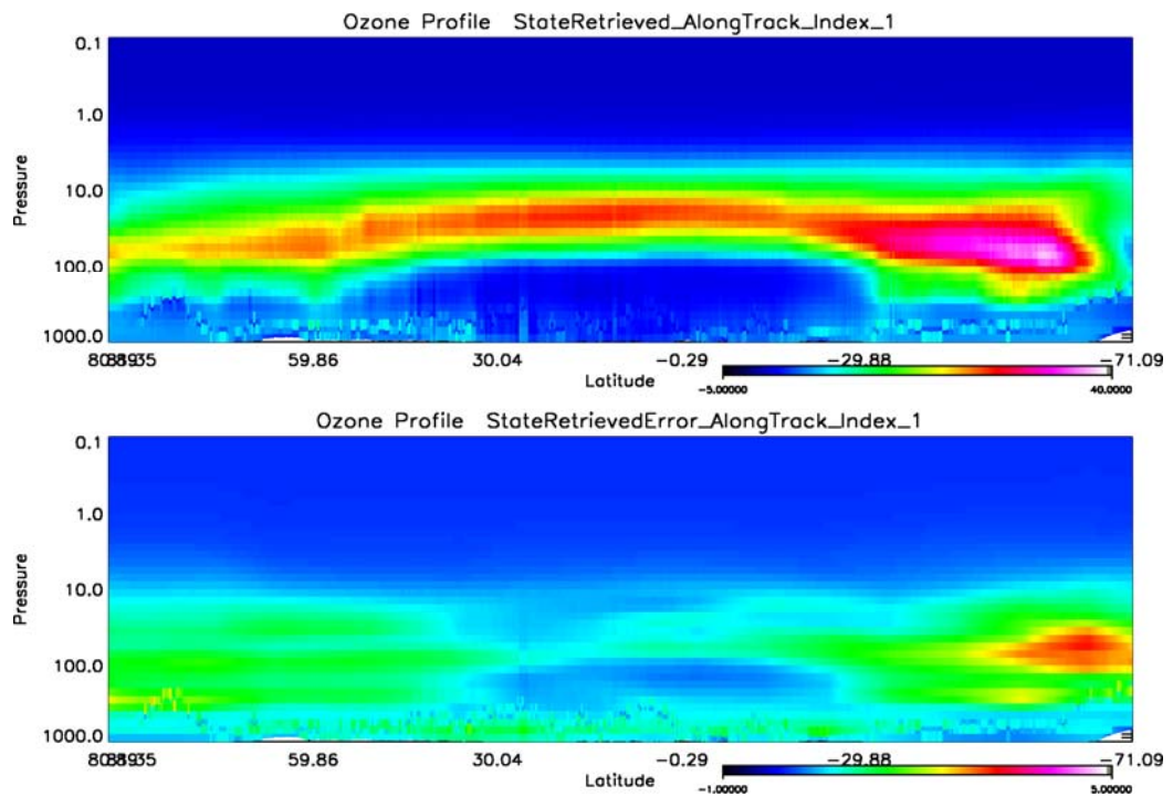
Figure 8: Retrieved ozone profile (top) and its retrieved error (bottom) for nadir swath in orbit 4679, indicated with letter (A). Instrument: GOME-2 on Metop-A.
