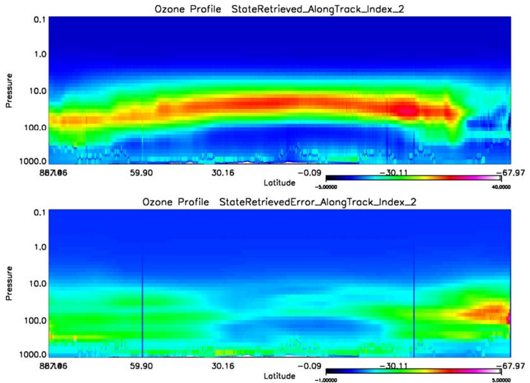
Figure 9: Retrieved ozone profile (top) and its retrieved error (bottom) for western swath of orbit 4683, indicated with letter (B). Instrument: GOME-2 on Metop-A.
