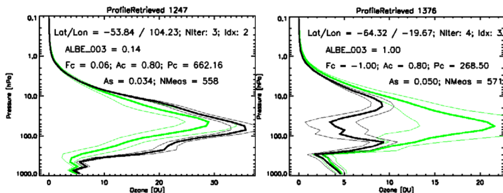
Figure 15: Retrieved ozone profiles (black), it's a priori (green) for retrieval in the ozone maximum in orbit 4679 (left), and in the ozone hole in orbit 4683 (right), indicated with the A and B. Instrument: GOME-2 on Metop-A.
