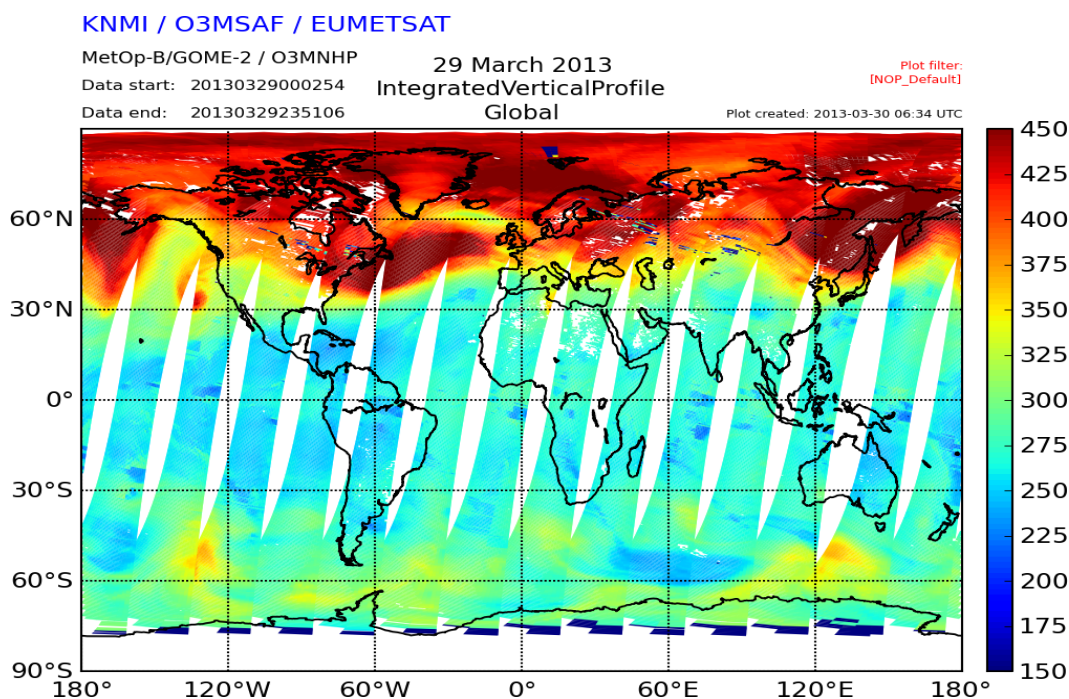
Figure 12: Integrated vertical ozone profile from GOME-2 on Metop-B, calculated as the sum of the retrieved profile on March 29 th 2013.
