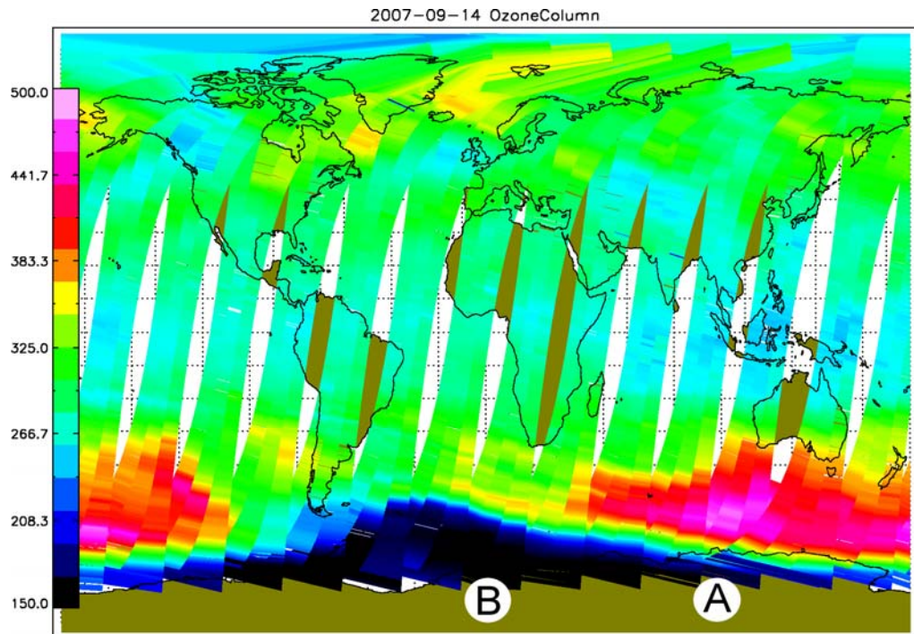
Figure 7: Total ozone column, calculated as the sum of the retrieved profile for September 14th 2007. Instrument: GOME-2 on Metop-A.
