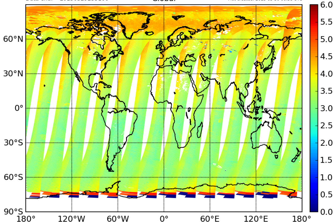
Figure 11: Degrees of Freedom for Signal for retrieved ozone profiles of GOME-2 on Metop-B on March 29 th 2013.
