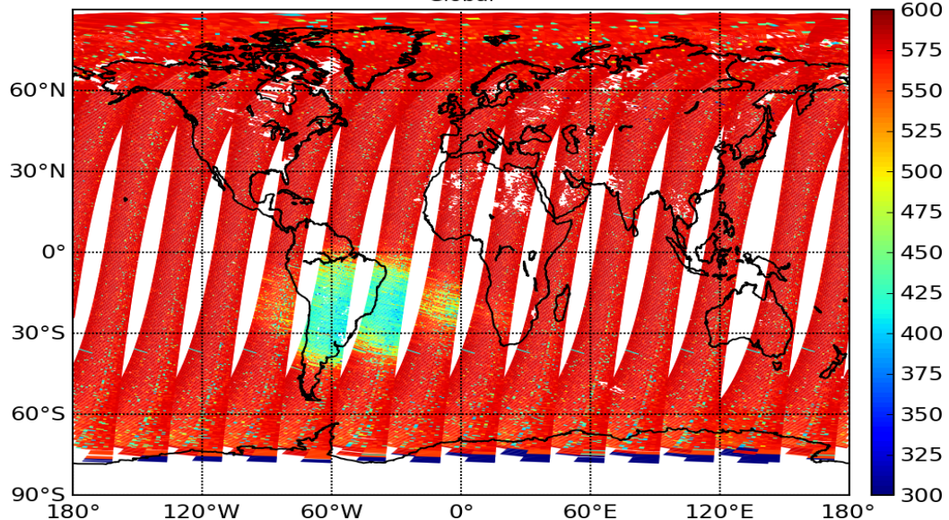
Figure 14: Number of spectral measurements of GOME-2 on Metop-B for each retrieved vertical ozone profile on March 29 th 2013.
