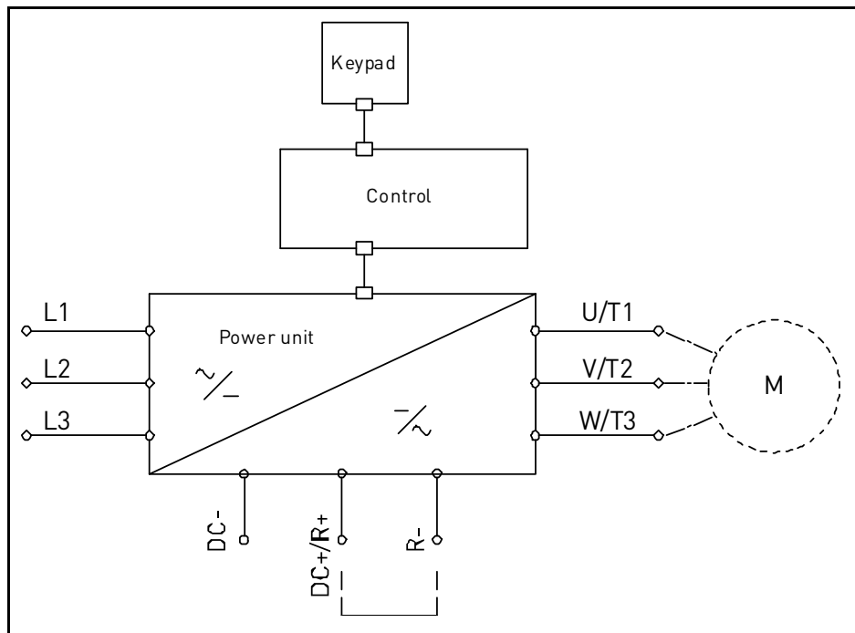
Figure 17. Principal connection diagram
