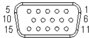
Figure 2.11 VGA Connector
