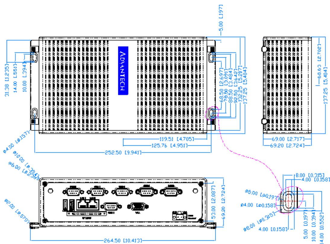
Figure 1.1 ARK-3360 Mechanical dimension drawing
