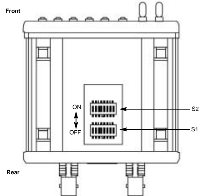
Figure 3. Underside of Model 2701/I, Showing Location of DIP Switches
