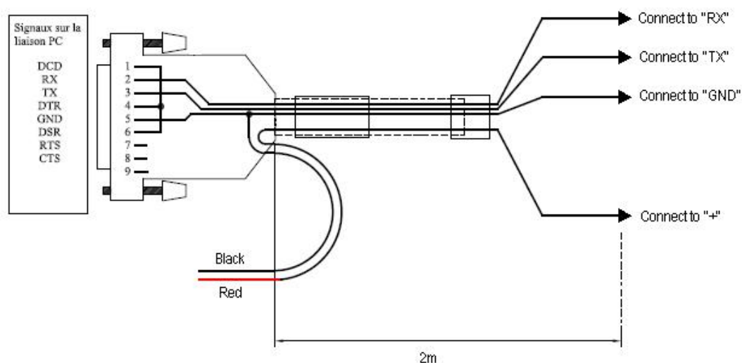
Internal SUBD9 connection
