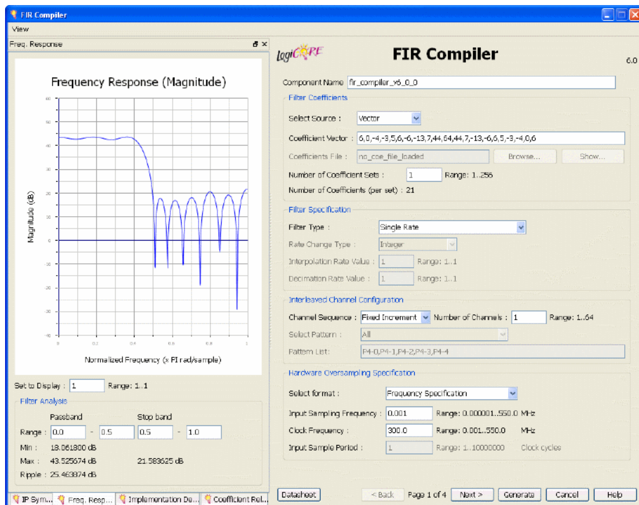
Figure 3-27: CORE Generator Interface
