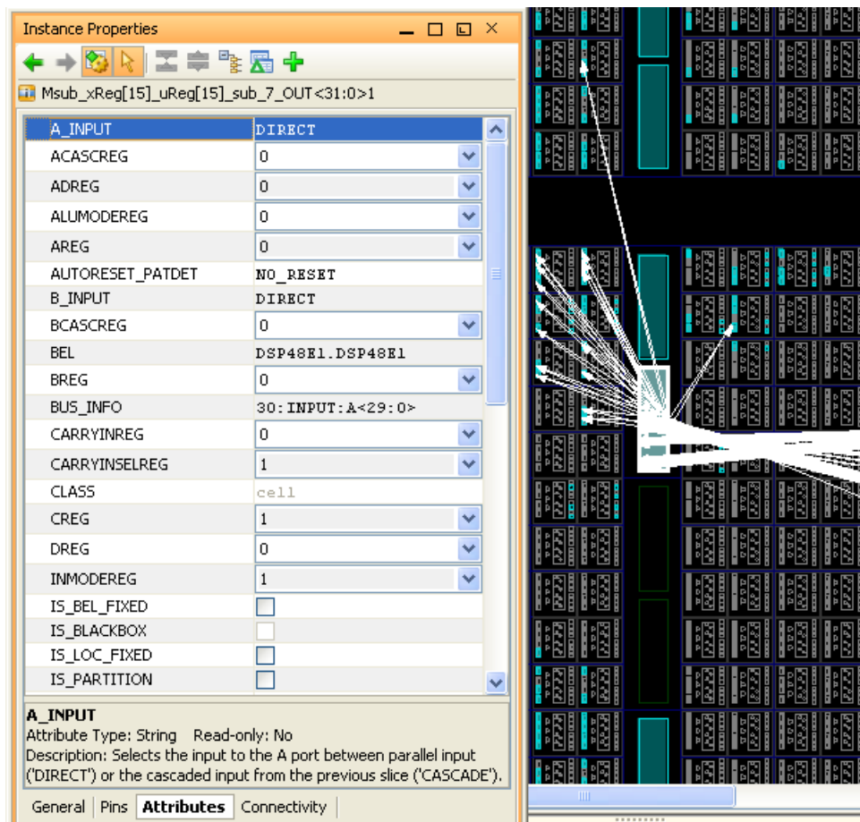
Figure 4-57: Properties View
