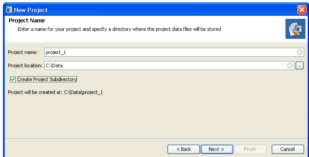
Figure 3-1: Create Project
