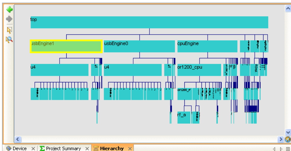
Figure 4-63: Hierarchy View
