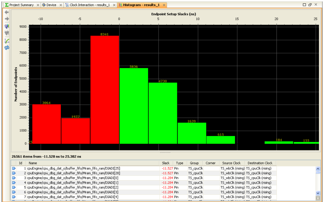
Figure 7-24: Slack Histogram
