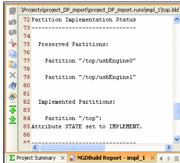
Figure 13-4: Viewing Partition Actions in NGDBuild Report
