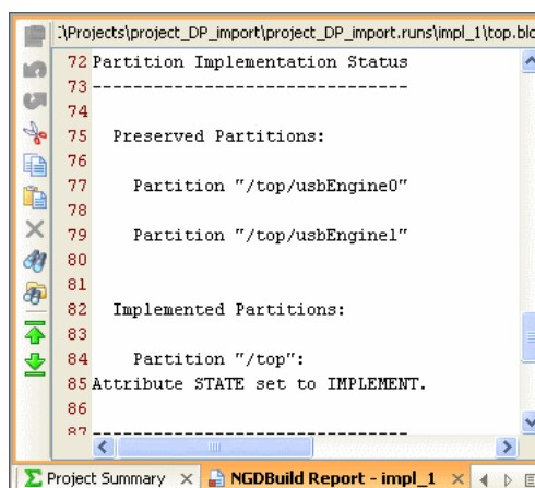
Figure 13-8: Partition Import Activity in the NGDBuild Report
