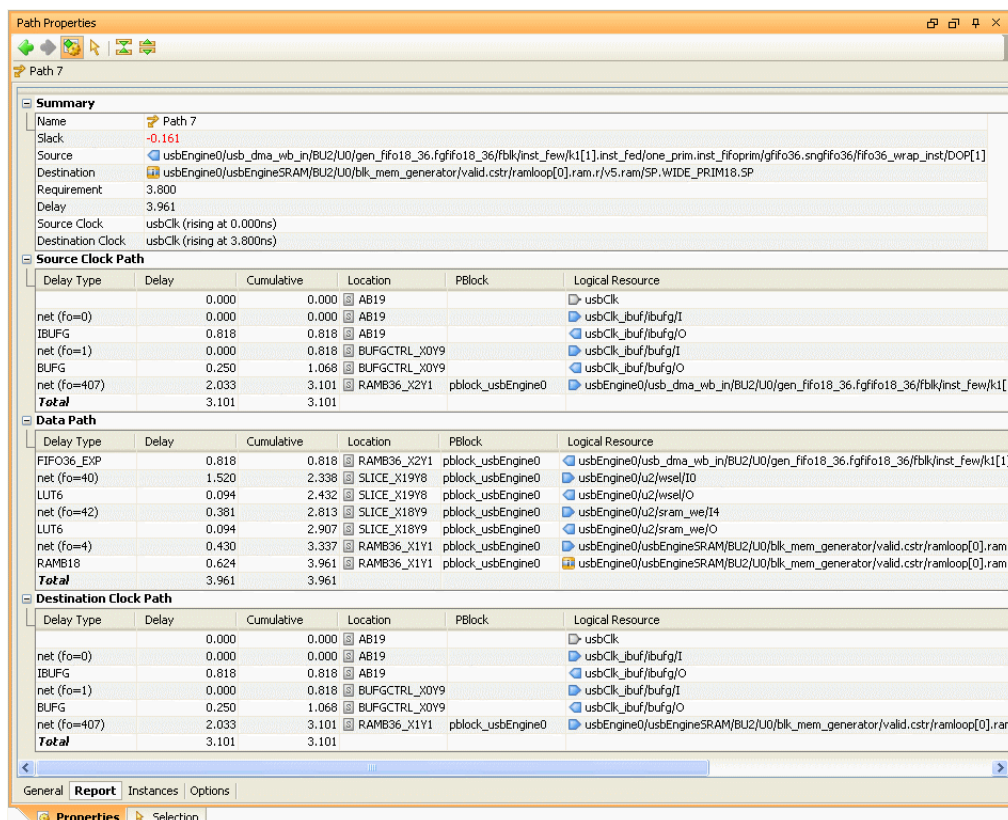
Figure 11-9: Path Properties View: Report Tab
