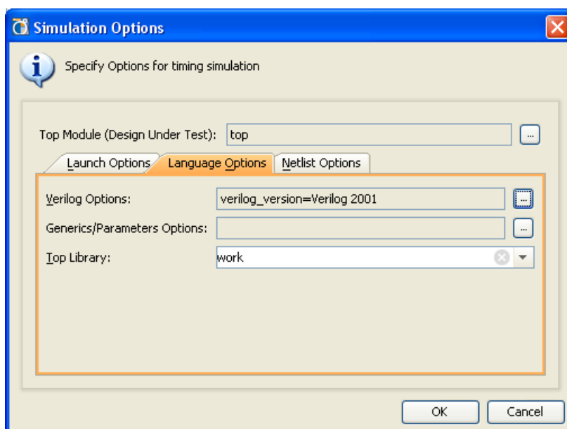
Figure 11-22: Timing Simulation Language Options
