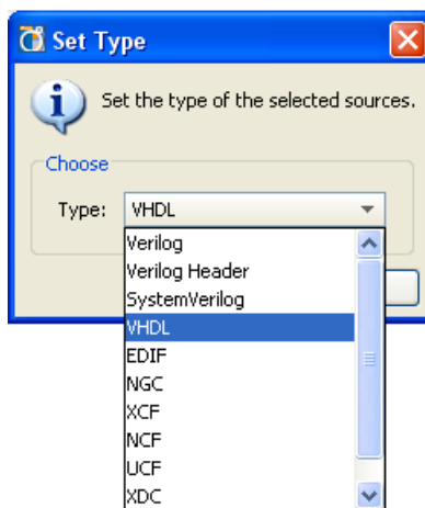
Figure 4-40: Set Type
