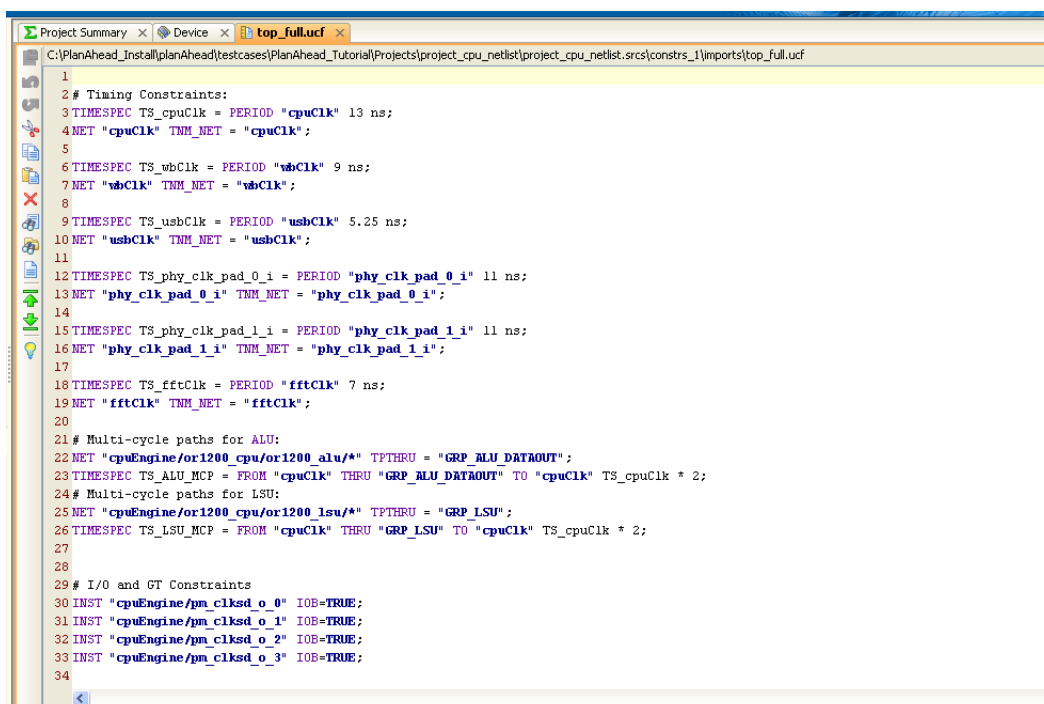
Figure 7-9: Text Editor
