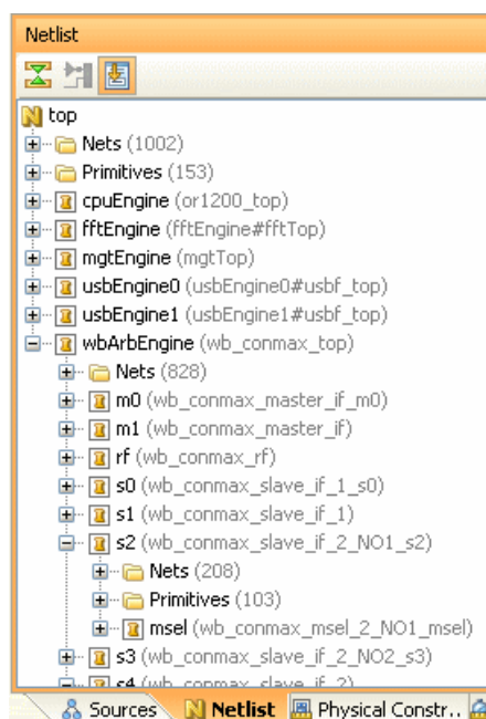
Figure 4-59: Netlist View
