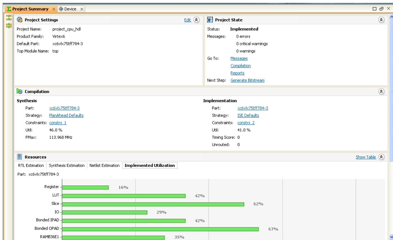
Figure 3-36: Project Summary
