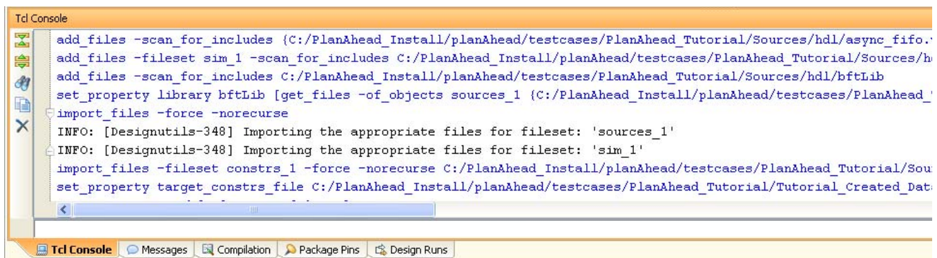
Figure 4-11: Tcl Console
