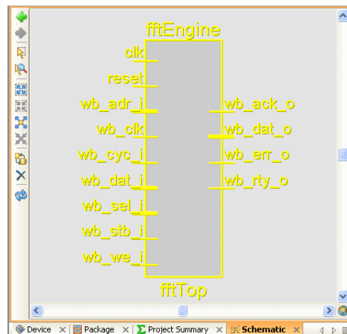
Figure 4-48: Schematic View
