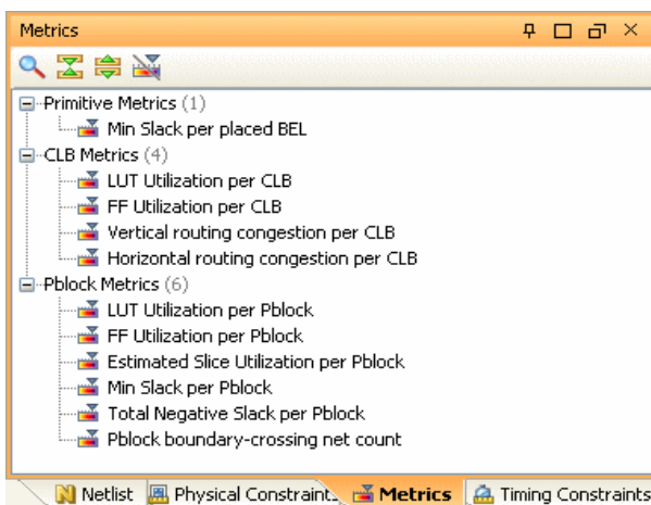
Figure 11-15: Metrics View
