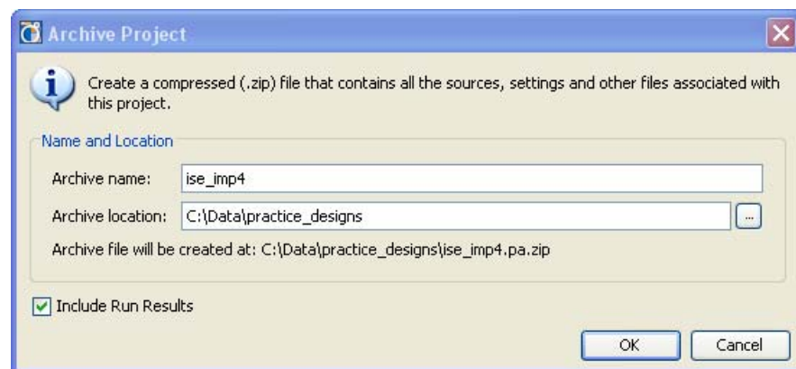
Figure 3-13: Archive Project
