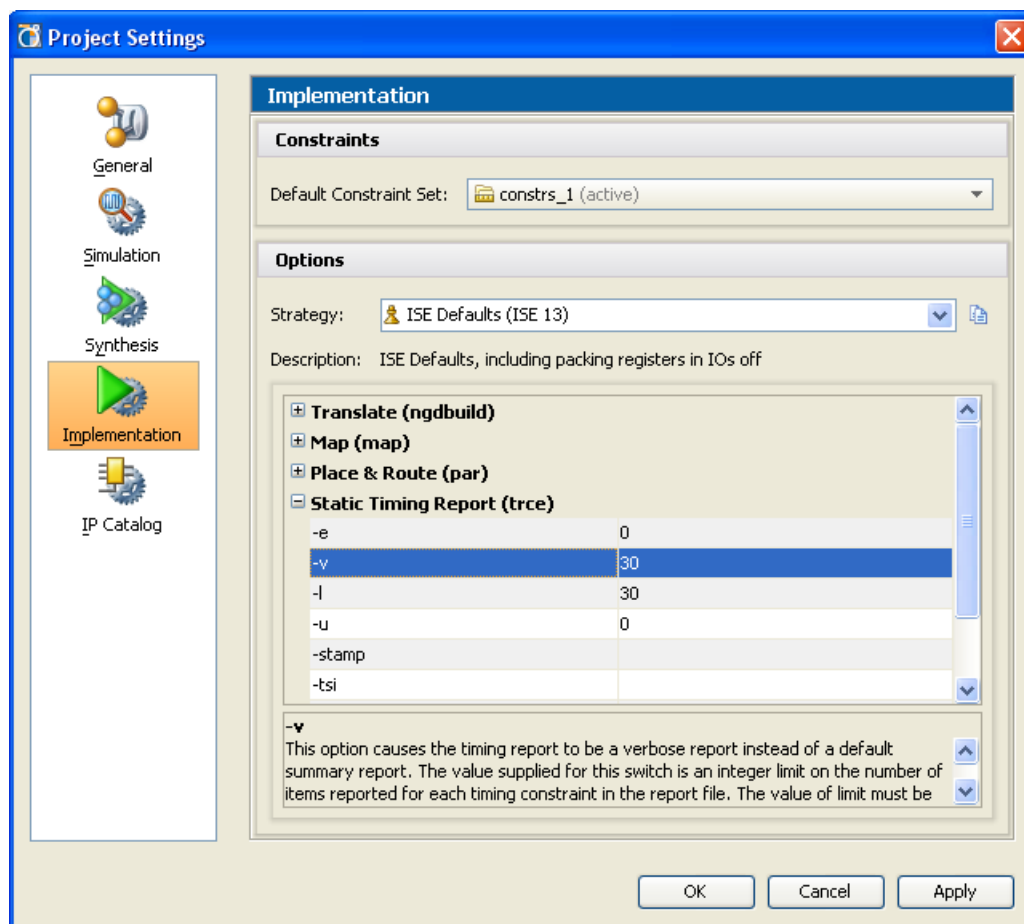
Figure 3-44: Implementation Project Settings
