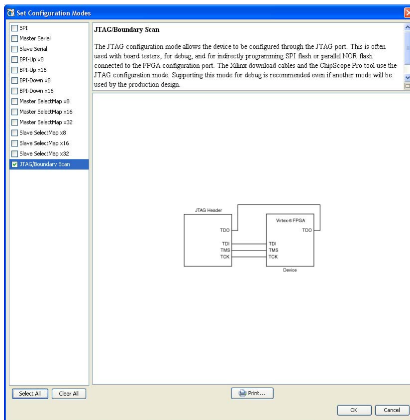
Figure 8-8: Set Configuration Modes Dialog Box
