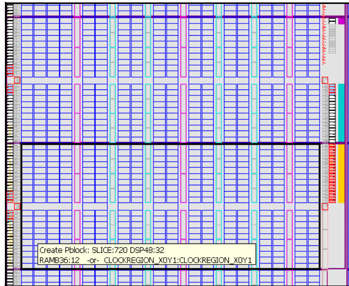
Figure 10-6: Creating Clock Region Pblocks
