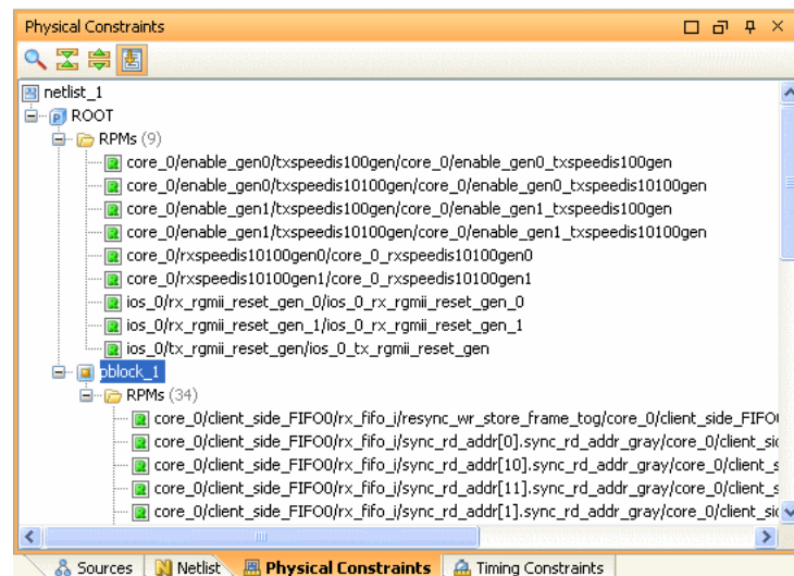
Figure 7-31: Displaying Relatively Placed Macros “RPMs”
