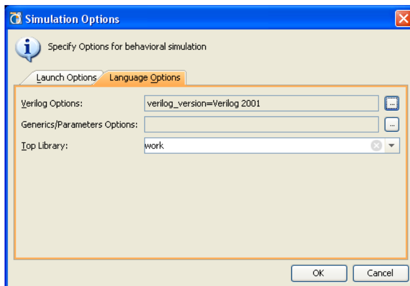
Figure 5-12: Behavioral Simulation Language Options
