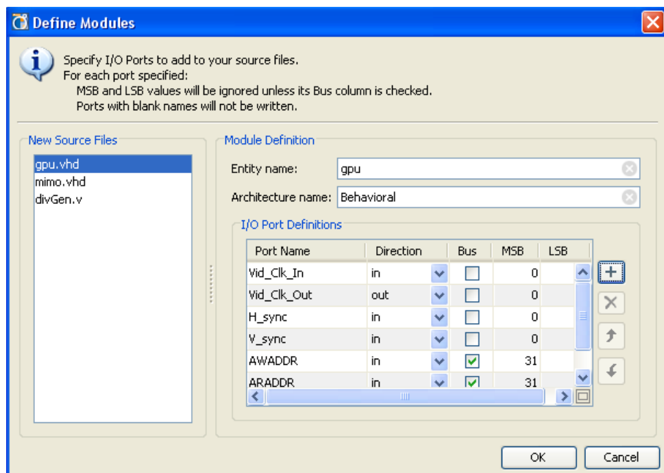
Figure 3-5: Define Modules Dialog Box
