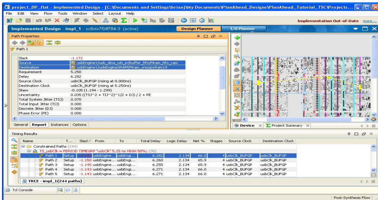
Figure 11-10: Highlighted Timing Paths in the Device View
