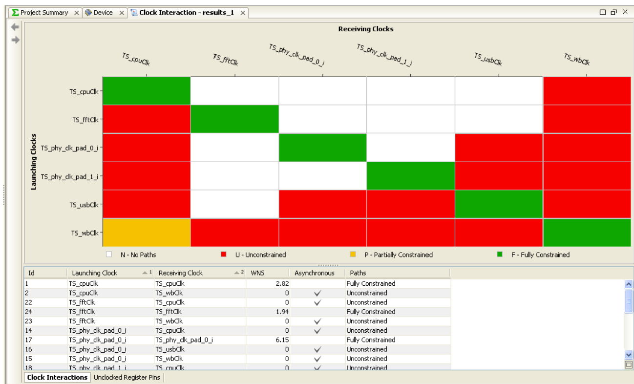
Figure 7-28: Clock Interaction Report
