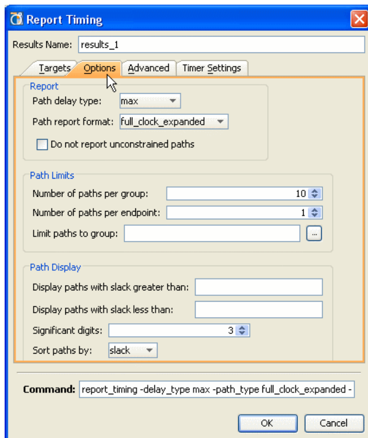
Figure 7-14: Report Timing - Options tab
