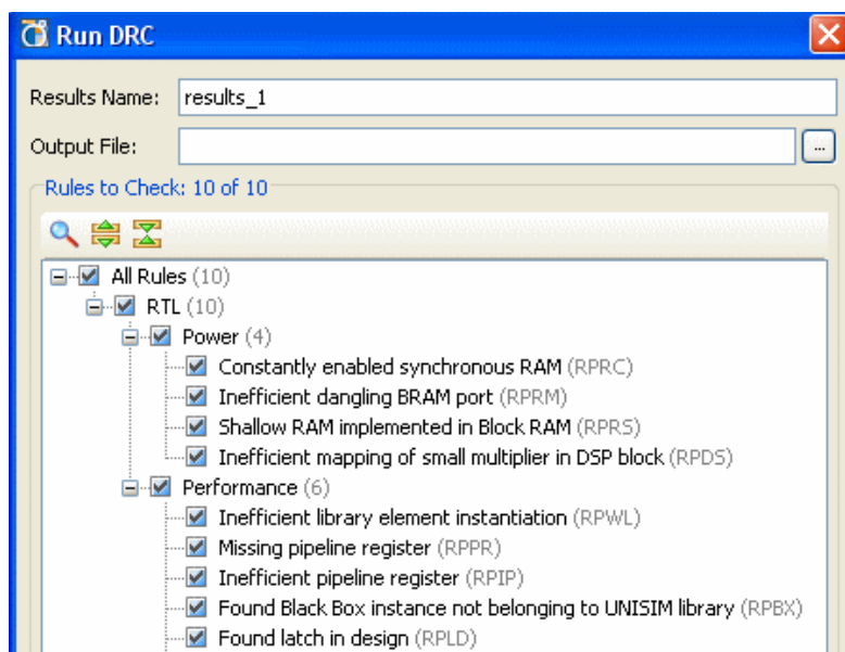
Figure 5-14: Run Design Rule Checker Dialog Box
