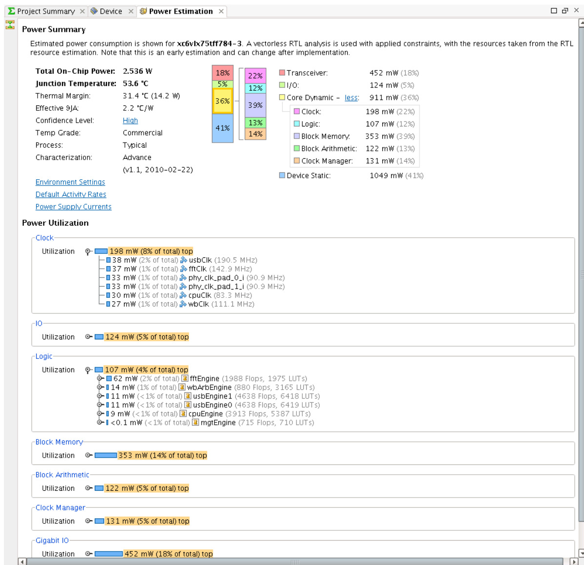
Figure 5-7: Power Estimation View
