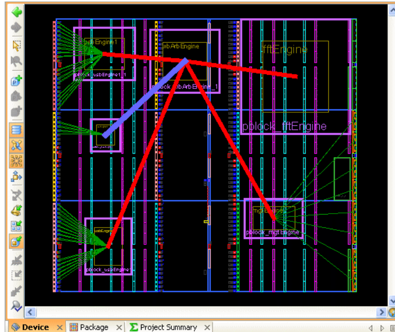
Figure 10-2: Pblock Connectivity Analysis in the Device View
