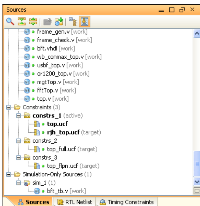
Figure 3-23: Setting the Active Constraint Set
