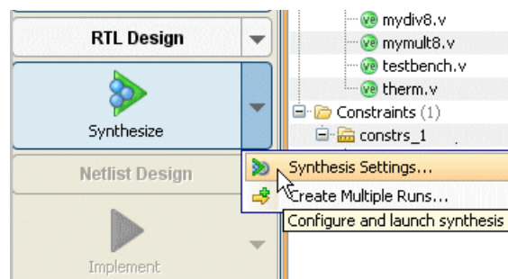
Figure 6-2: Configuring Synthesis Run Settings
