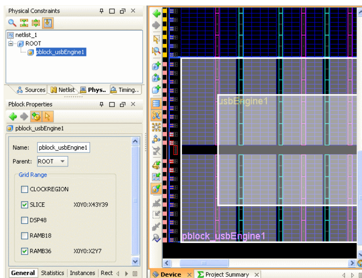
Figure 10-11: Pblock Shading Reflects Logic Contained in Pblock
