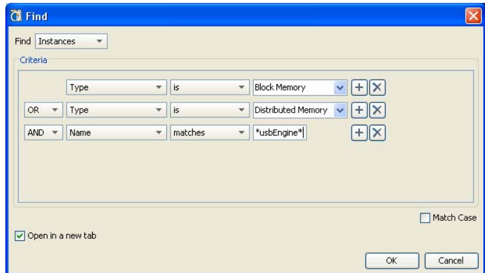
Figure 4-32: Searching for Objects with Additional Search Criteria
