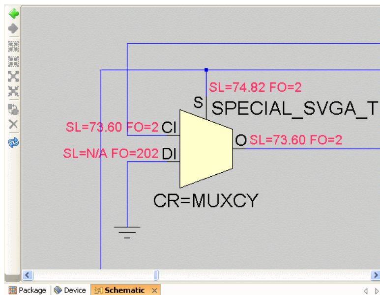
Figure 4-53: Annotated Pins in the Schematic View
