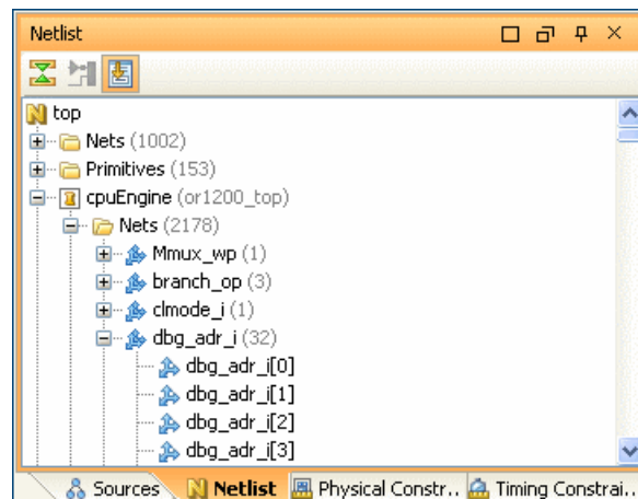
Figure 4-61: Nets Folder in Netlist View
