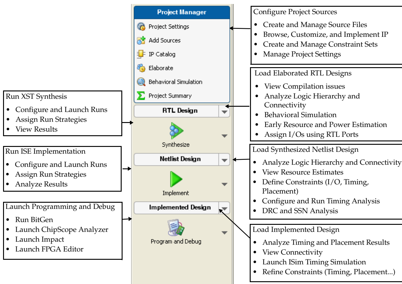
Figure 2-2: PlanAhead Software Flow Navigator - RTL Project
