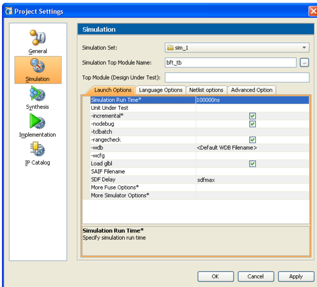
Figure 3-42: Simulation Project Settings
