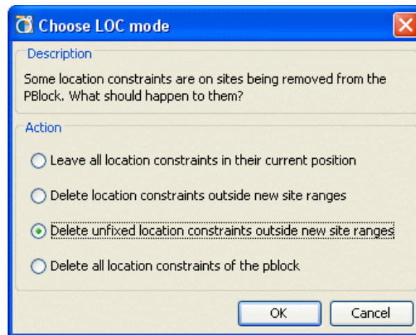
Figure 10-13: Setting Behavior for Modifying Pblocks with LOCs
