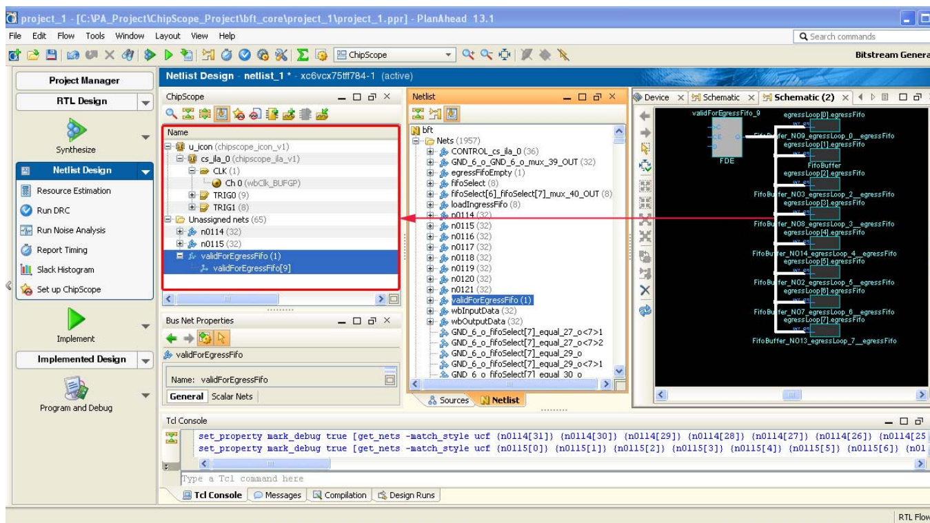
Figure 12-8: Dragging and Dropping Nets onto Debug Core Ports
