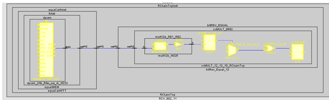
Figure 4-56: Logic Hierarchy in Schematic View
