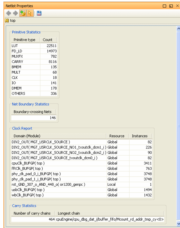
Figure 7-4: Netlist Resource Statistics
