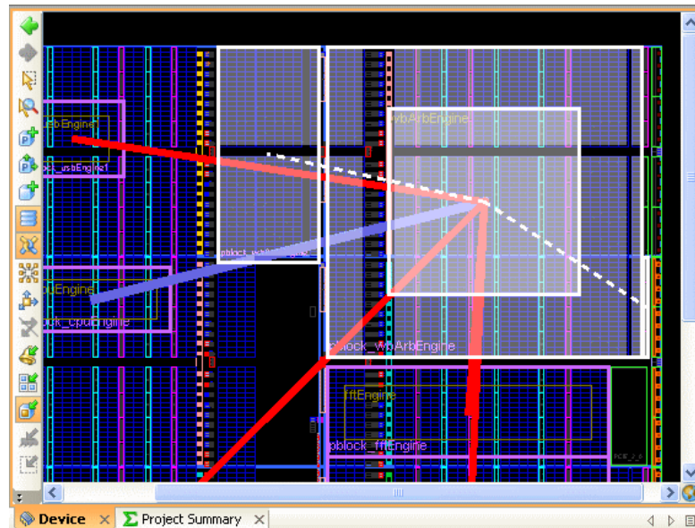
Figure 10-5: Creating Pblocks with Non-Rectangular Shapes
