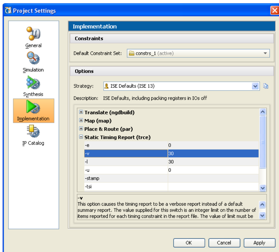
Figure 9-1: Implementation Project Settings
