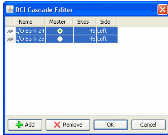
Figure 8-15: Creating a DCI Cascade
