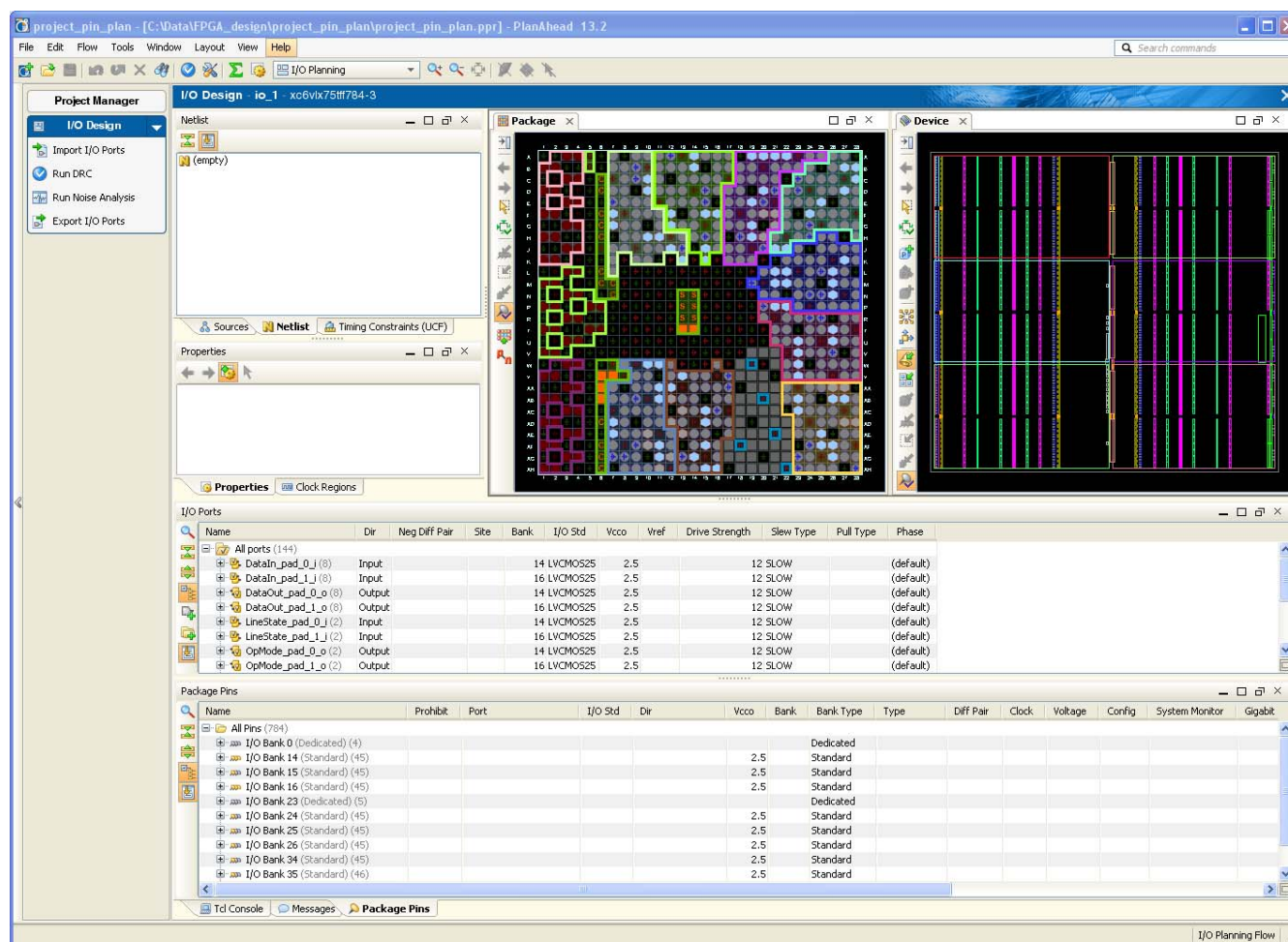
Figure 8-1: I/O Planning Environment
