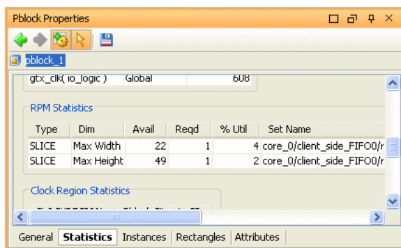
Figure 7-32: RPM Utilization Statistics for Pblocks
