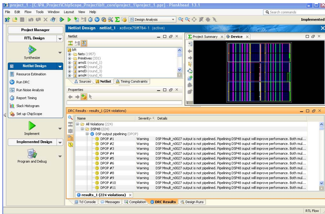
Figure 7-34: DRC Results
