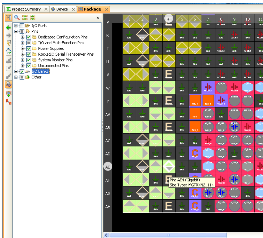
Figure 4-46: Package View
