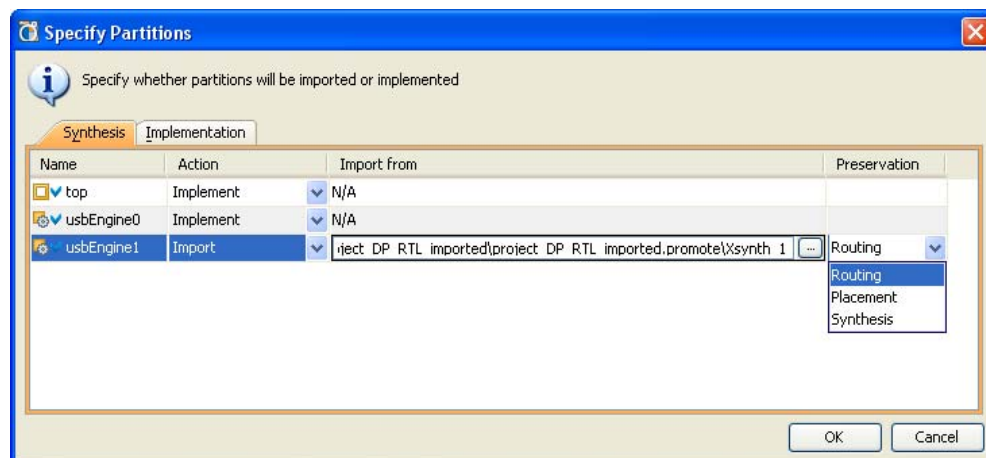
Figure 13-7: Importing Partitions
