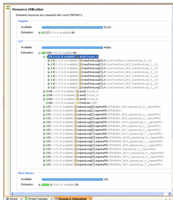
Figure 7-2: Hierarchical Resource Estimation
