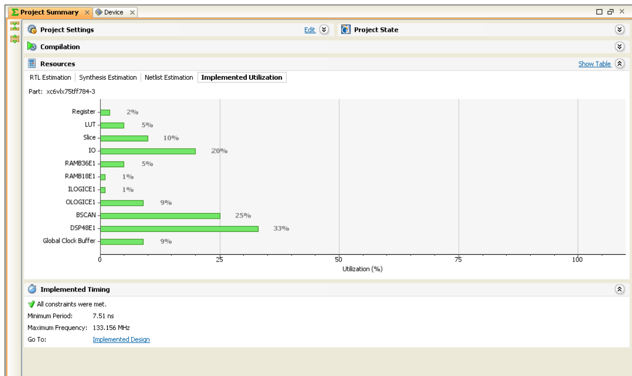
Figure 3-37: Graphical Resource Estimates
