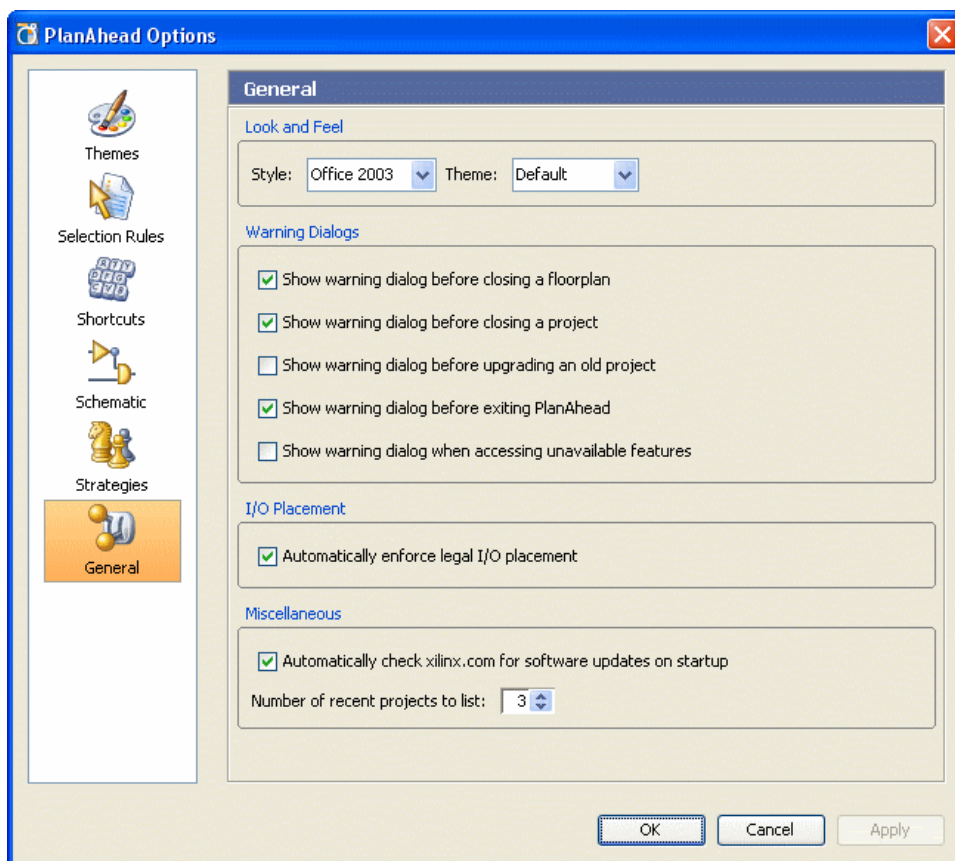
Figure C-1: Automatically Check xilinx.com for Software Updates
