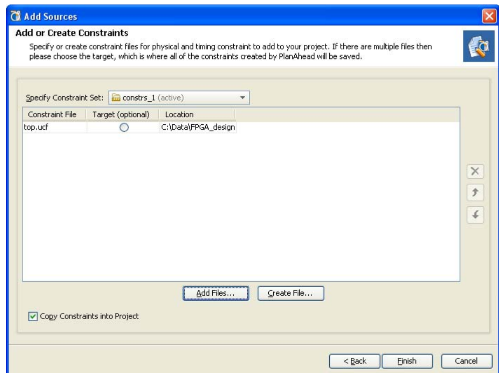
Figure 3-20: Adding Constraint Files using Add Sources
