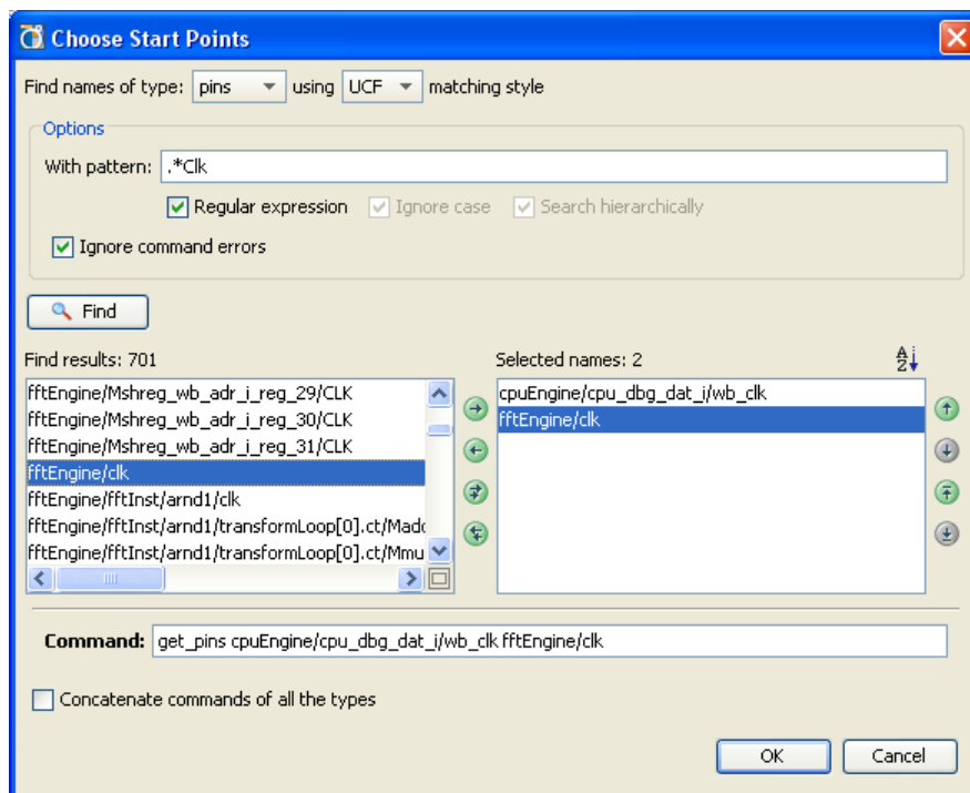
Figure 7-13: Choose Start Points Dialog Box
