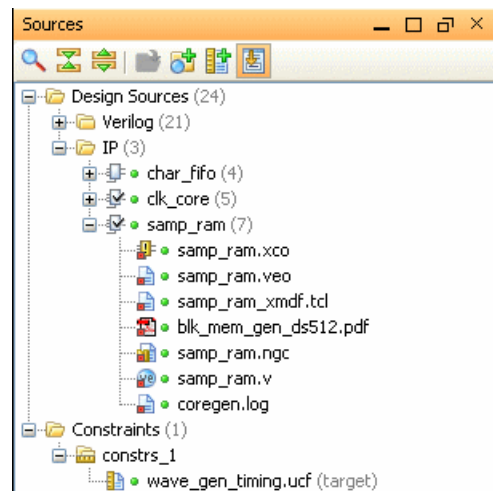
Figure 3-29: IP Displayed in Sources View
