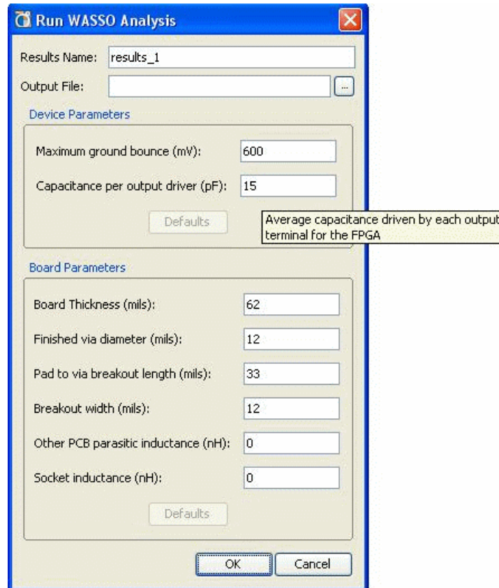
Figure 8-35: Run WASSO Analysis Dialog Box
