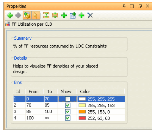
Figure 11-16: Properties View: Set Metric Range Values
