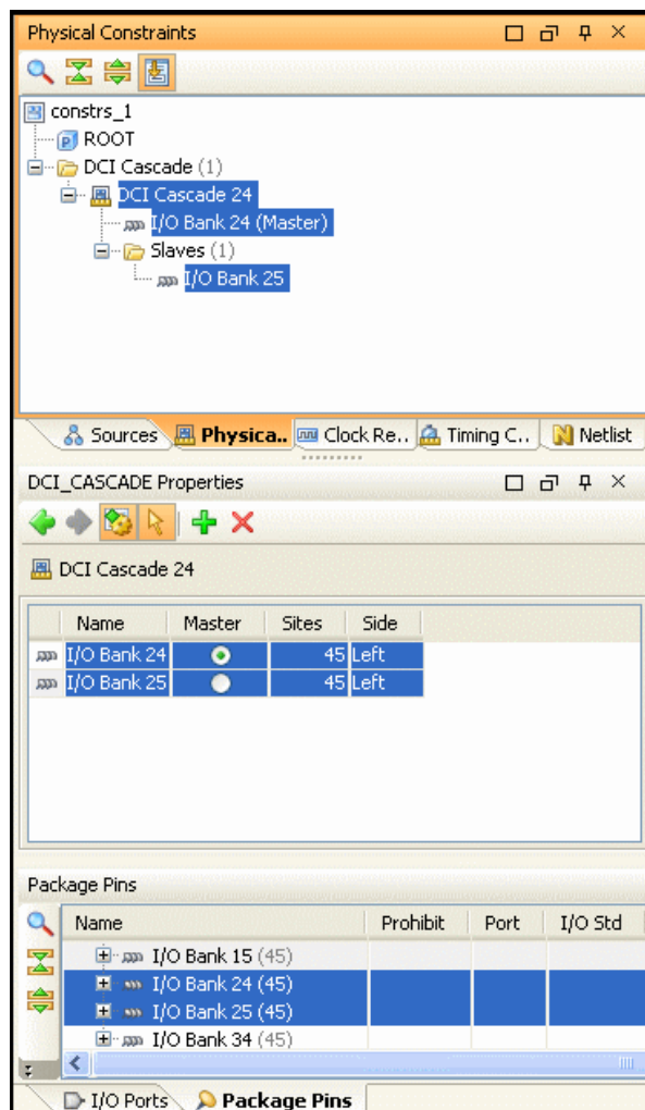
Figure 8-16: Viewing DCI Cascades
