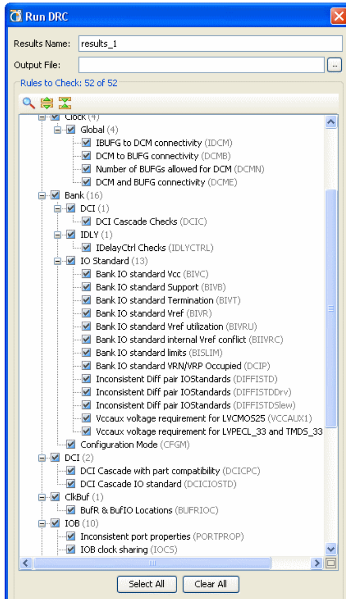
Figure 8-27: Run DRC Dialog Box: I/O Pin and Clock DRC Rules
