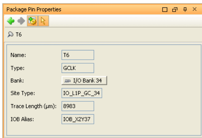
Figure 8-2: Package Pin Properties
