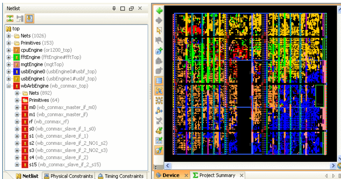
Figure 11-14: Matching Highlighting Color in the Netlist and Device Views
