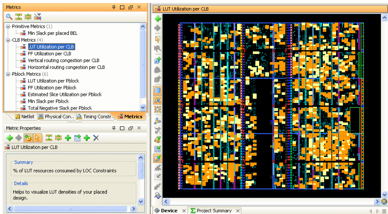
Figure 11-17: Metric Map in the Device View
