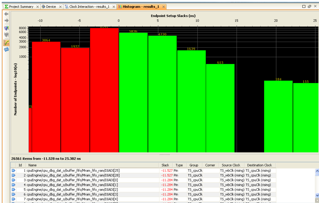
Figure 7-25: Slack Histogram - Log10 scale
