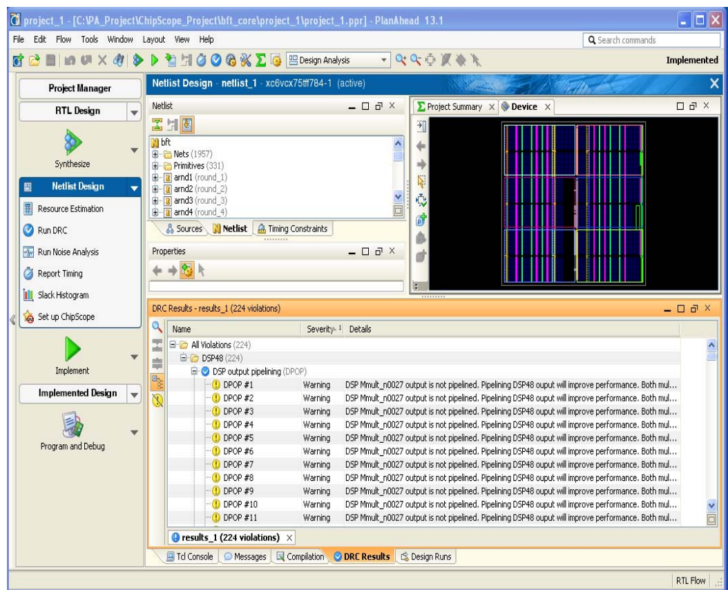
Figure 5-15: RTL Design with Objects that Violate DRCs
