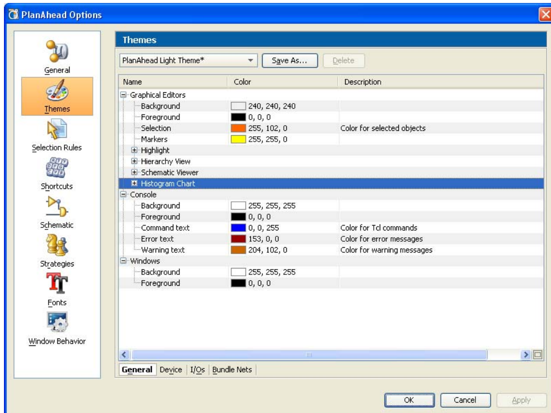
Figure 4-70: Theme Options
