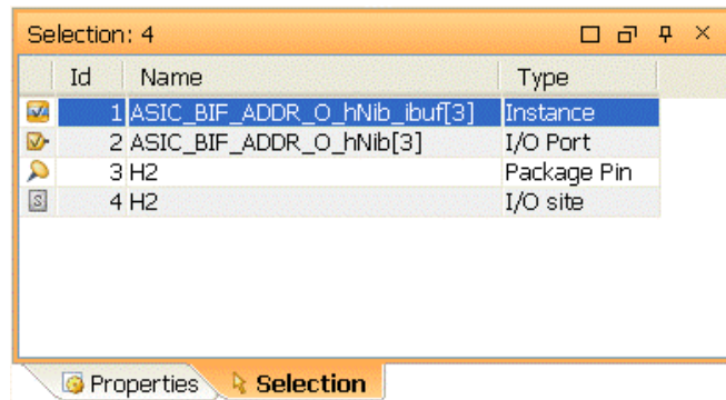
Figure 4-28: Selection View
