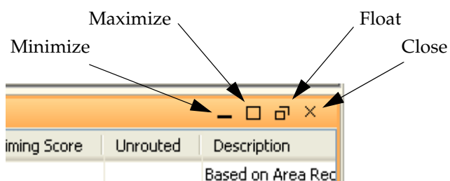
Figure 4-3: Window Controls
