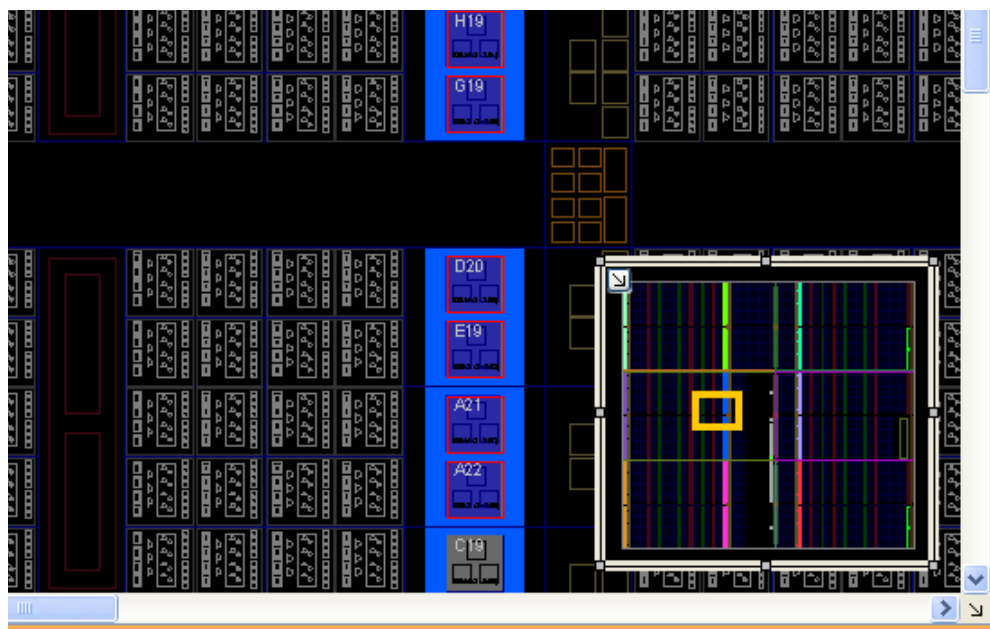
Figure 4-16: World View
