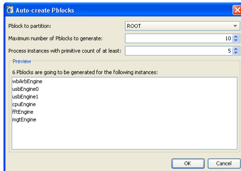
Figure 10-19: Auto-Create Pblocks
