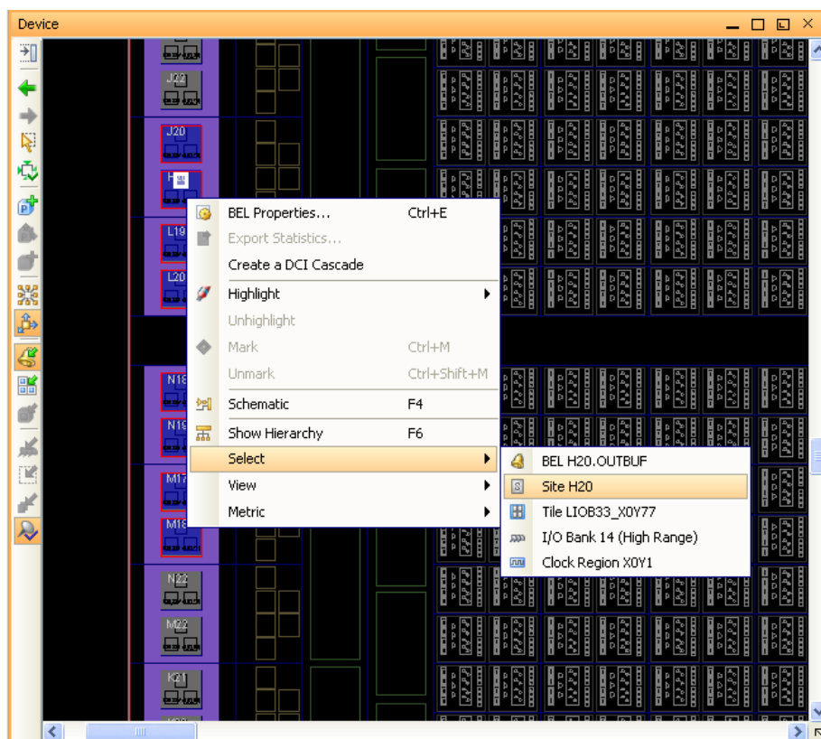
Figure 4-25: Select > Objects
