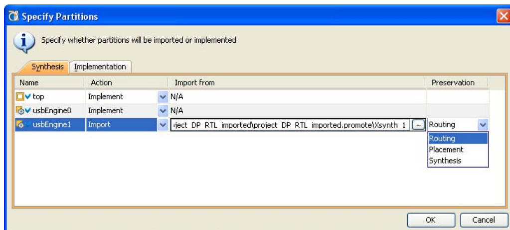
Figure 13-3: Specify Partitions
