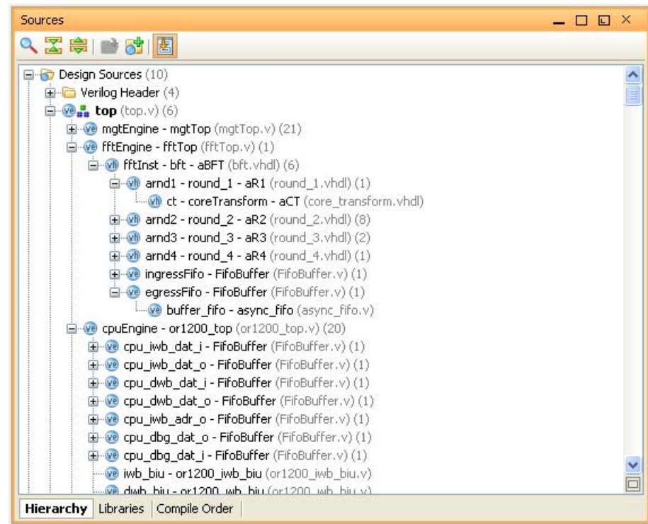
Figure 4-39: Sources View
