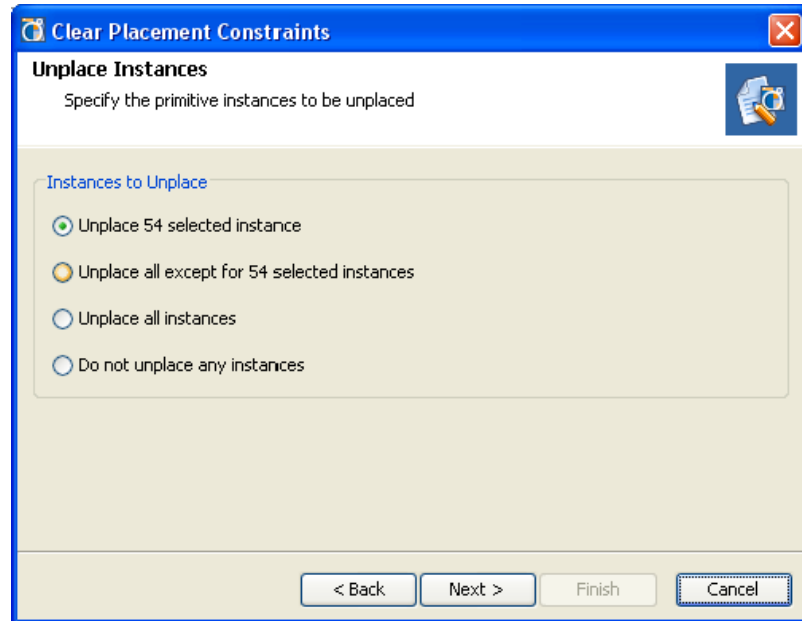
Figure 10-26: Unplace Instances
