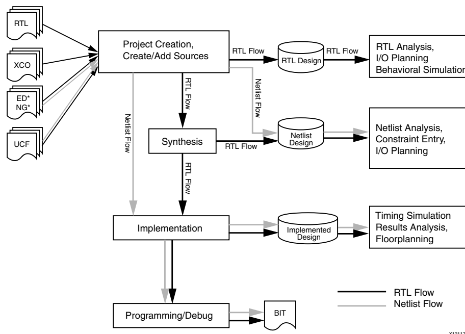
Figure 2-1: PlanAhead Design Flows
