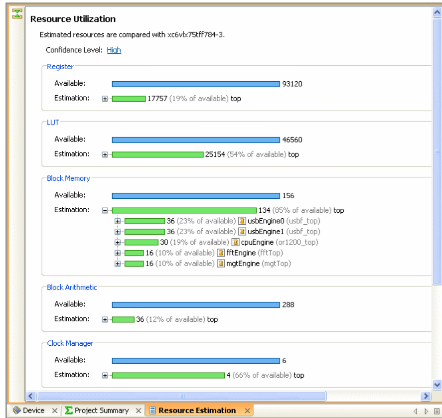
Figure 5-3: Resource Estimation View for the RTL Design
