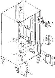
Cabinet 5.09
