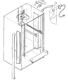
Cabinet 5.07
