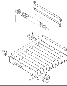
Candy Shelf 5.19
