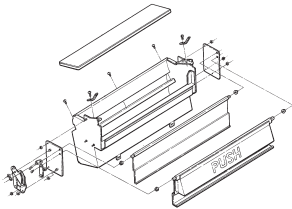
Delivery Bin 5.25
