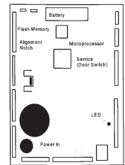
Logic Board 5.15
