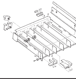
Convertible Shelf 5.21
