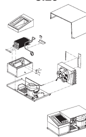
Chill Machine Supplement 5.29
