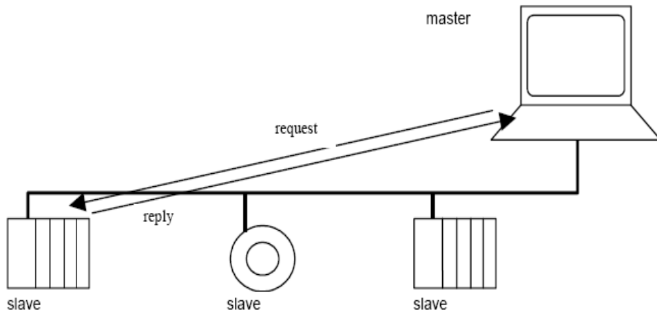
Figure 1 MODBUS Network
