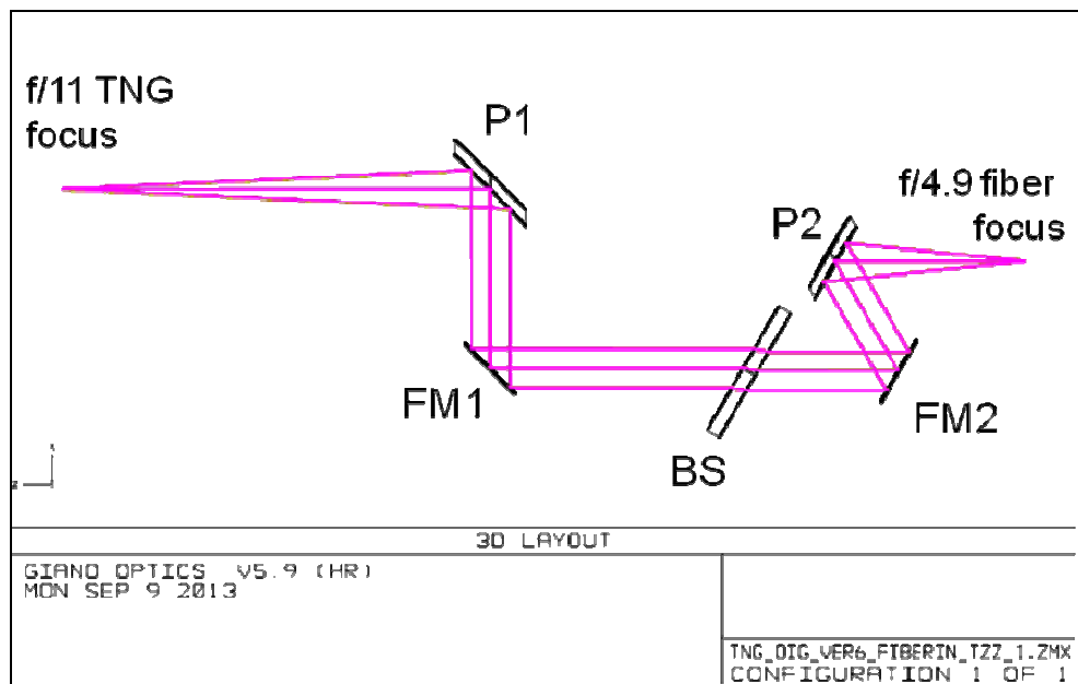
Fig. 7 Zemax optical design of the downstream mode. P1 and P2 are commercial parabolae, BS is the dichroic beamsplitter, FM are folding mirrors. (File: TNG_oig_ver6_fiberin_tzz_1.zmx)
