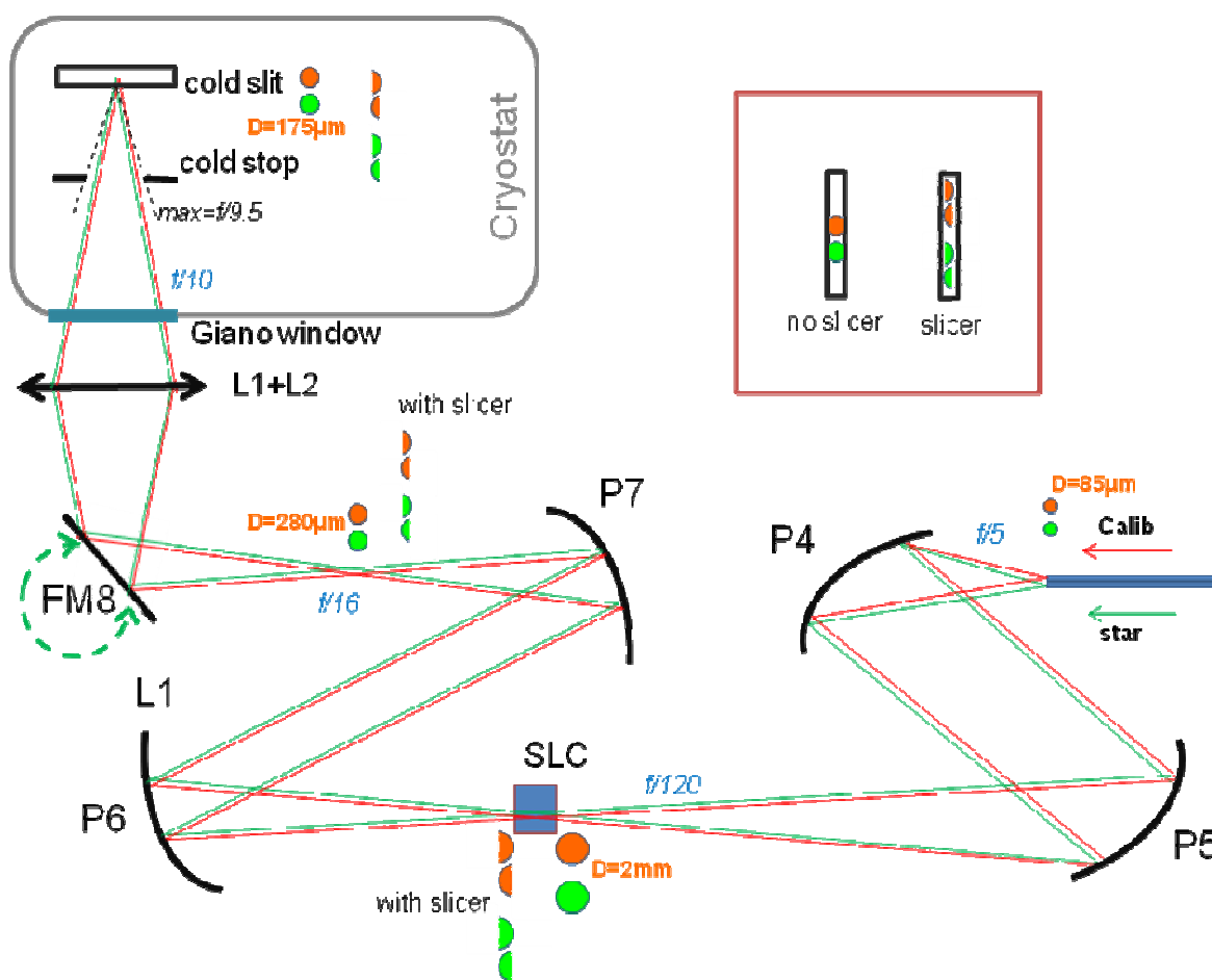
Fig. 22 Schematic representation of the Fiber-Spectrometer interface, assembled into the Preslit Giano Box. P4-P7 are Parabolic mirrors, FM8 is the rotator folding mirror, SLC the slicer. In the top right red box the matching between the slit and the foci is represented in case the slicer is used or not used.
