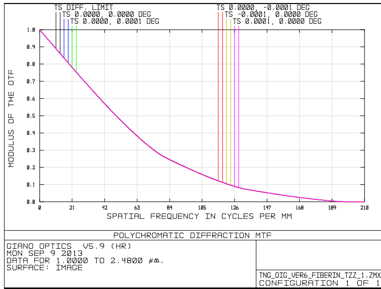
Fig. 8 MTF of the fiber in optical path
