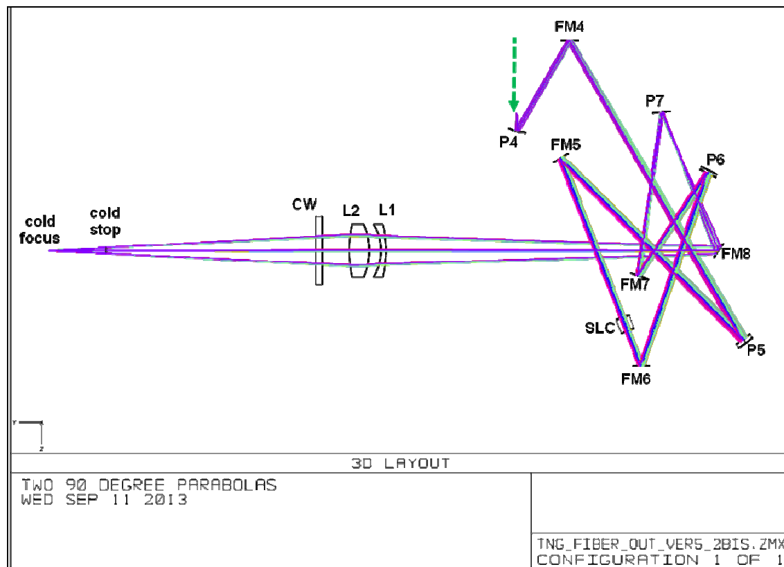
Fig. 25 Zemax optical design for the Preslit Giano Box. P are commercial parabolas.
