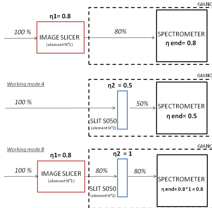
Fig. 30 The efficiency of Giano is increased by the use of the Slice Image: working in B modality the total efficiency is 0.8 with respect 0.5 of A modality.
