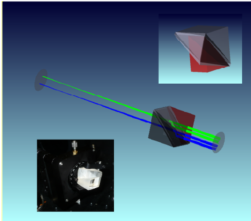
Fig. 31 The Image Slicer of the Giano's preslit, based on a Bowen Wallraven prism.
