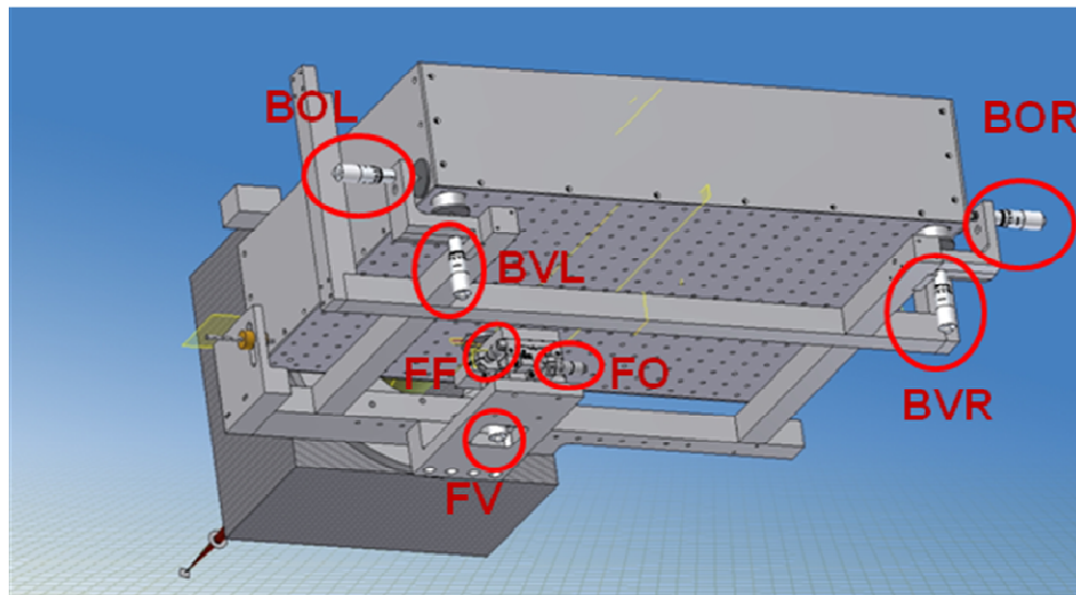
Fig. 24 Alignment details of the Preslit GIANO box. External micrometers are visible and for each ones the correct nominal position is given in Tab. 6
