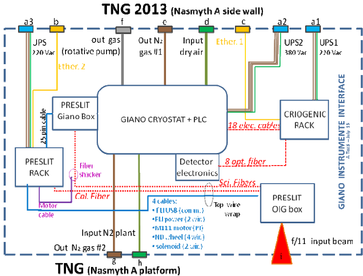
Fig. 16 Giano general interface scheme: electrical (blue and yellow perimetric boxes), gas (grey, brown and green boxes) and light (red) . The Giano instrumente internal cabling is represented, too.
