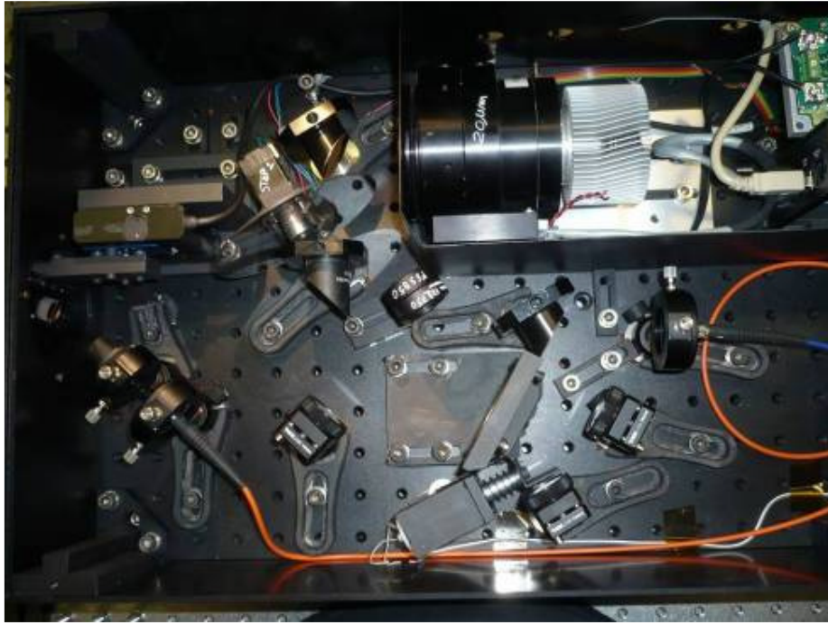
Fig. 2 Optics of the Preslit OIG box.
