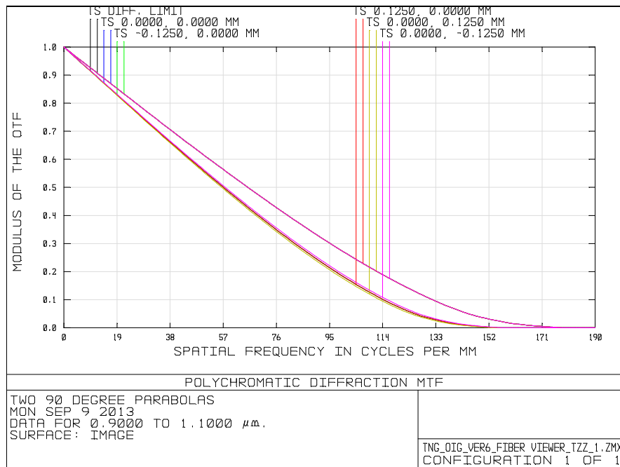
Fig. 13 MTF of the Fiber Viewer system optics
