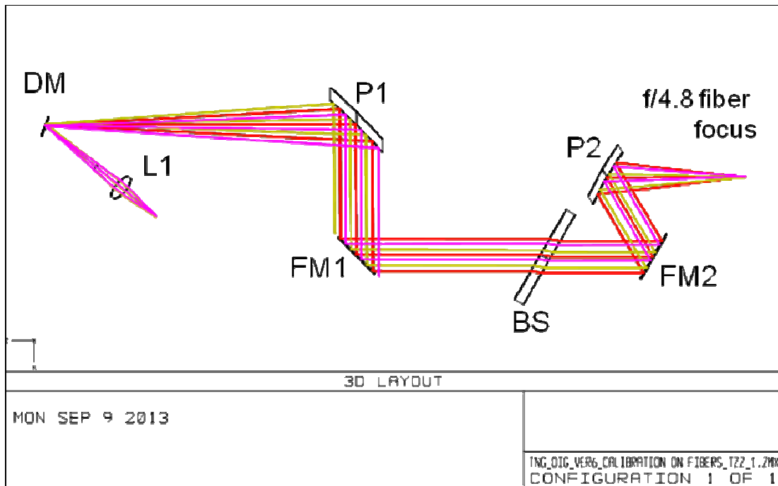
Fig. 9 Zemax optical design for the Calibration mode. P1 and P2 are commercial parabolas, BS is the dichroic beamsplitter, FM are folding mirrors, DM is D shape couple of mirrors remotely controlled.
