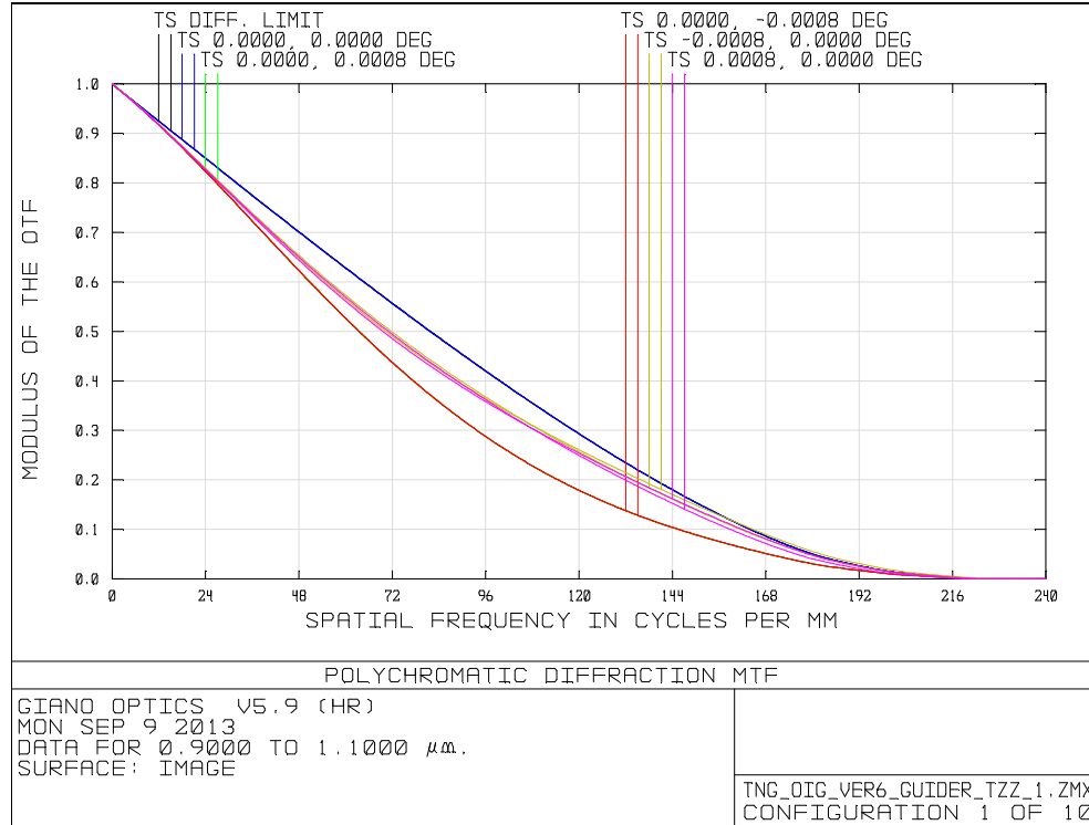
Fig. 11 MTF of the guider system optics
