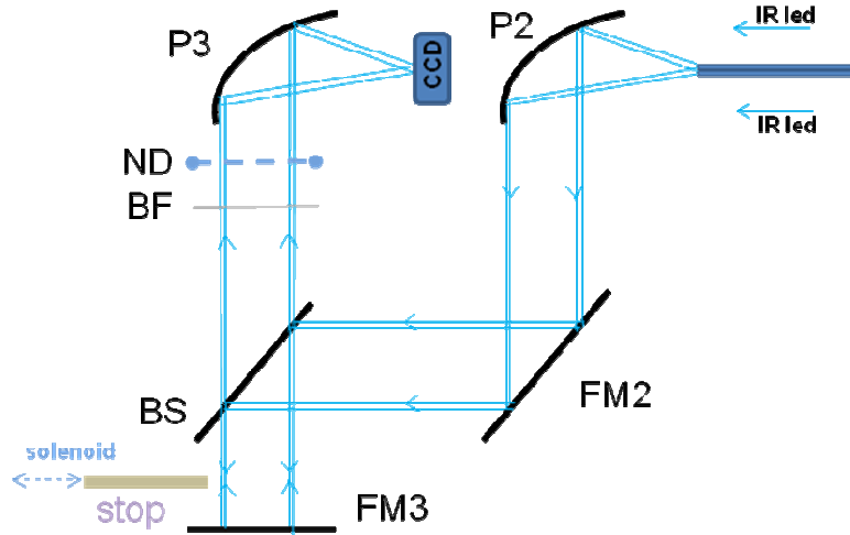
Fig. 6 Conceptual plot of the Preslit OIG box in the upstream modality. P3 is an identical off axis parabola as P2.
