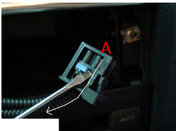
Step 4 : Eject the original optical input cable A (the one has light)
