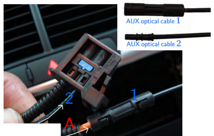
Step 5 : Connect the original optical input cable A (ejected in step 4) to the affiliated AUX optical connector 1. Insert the affiliated AUX optical cable 2 to original input.
