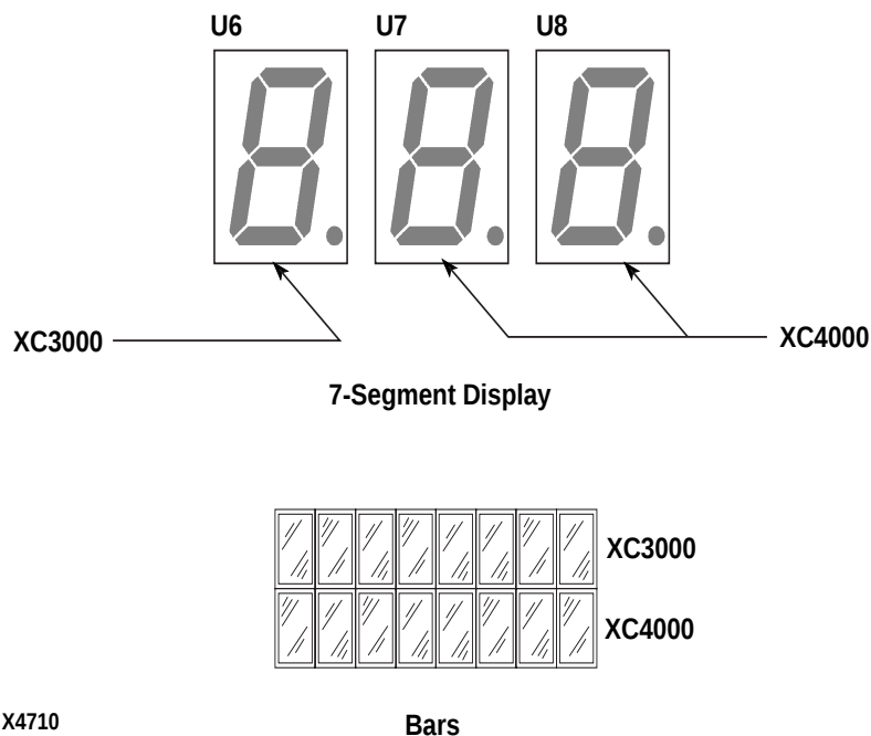
Figure 3-1 FPGA Demonstration Board Displays
