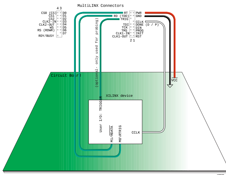
Figure 2-13 Verification of Configuration Data Only (XC3000)
