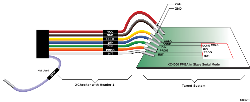
Figure 1-11 XChecker Connections to XC4000 Device
