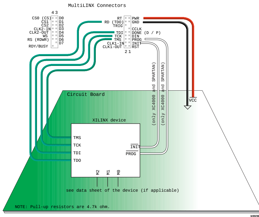
Figure 2-6 JTAG Mode (XC9000, Virtex, Spartan, XC5200, XC4000)
