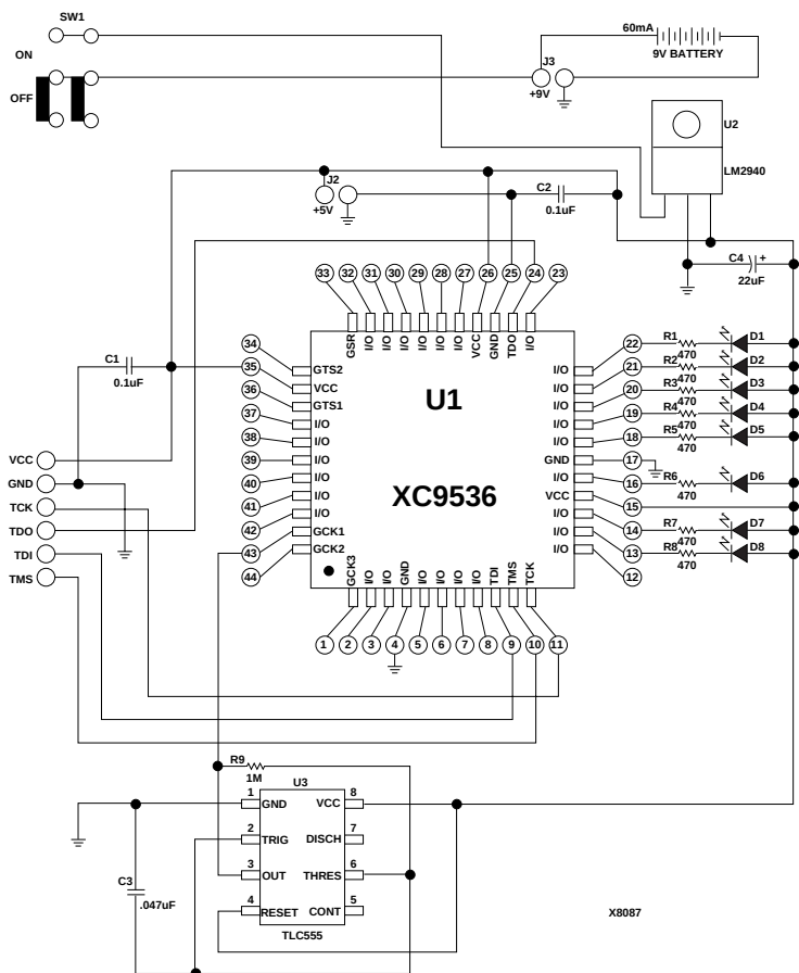
Figure 4-1 XC9536 Device Schematic
