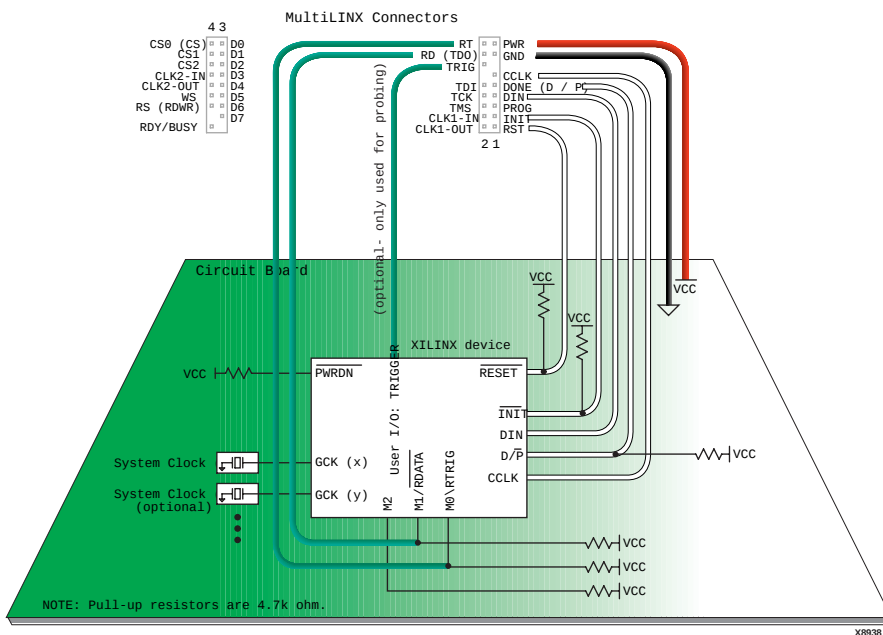
Figure 2-7 Slave Serial Mode (XC3000)
