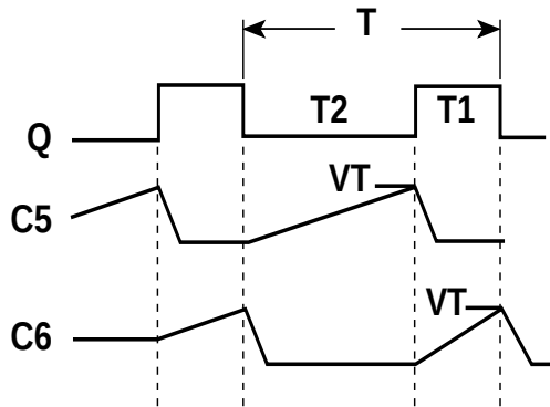
Figure 3-10 RC Network Waveforms
