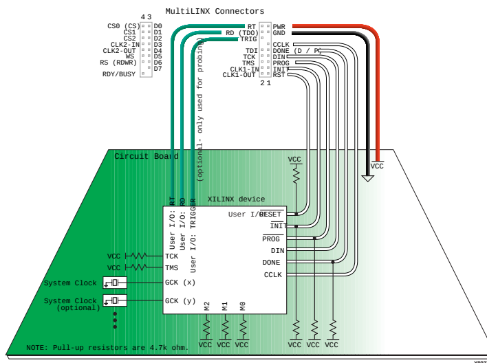
Figure 2-8 Slave Serial Mode (Spartan, XC5200, XC4000)
