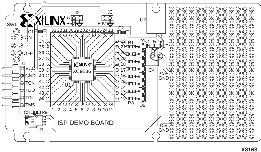
Figure 4-2 CPLD ISP Demonstration Board
