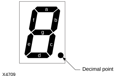
Figure 3-5 Seven-Segment Display
