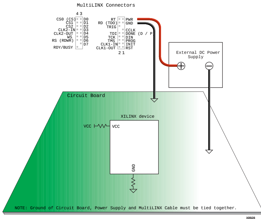
Figure 1-3 Optional External Power for the MultiLINX Cable
