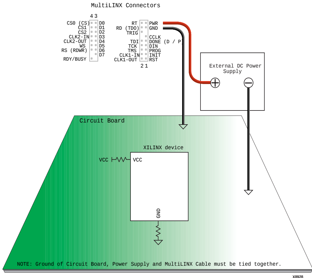
Figure 2-2 Optional External Power for the MultiLINX Cable
