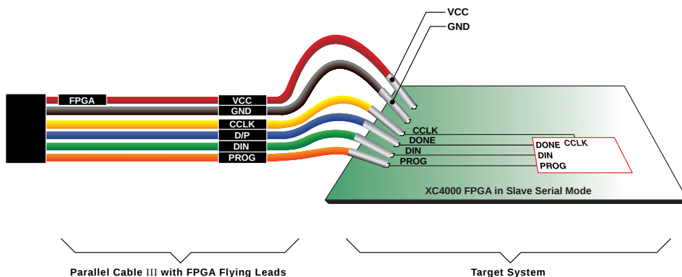
Figure 1-7 Parallel Cable III Connections to XC4000 Device
