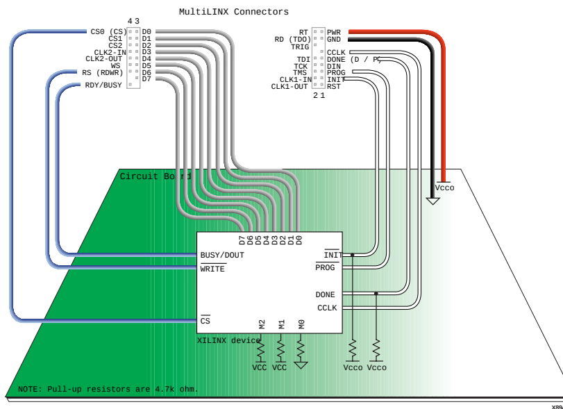
Figure 2-5 SelectMAP Mode (Virtex)
