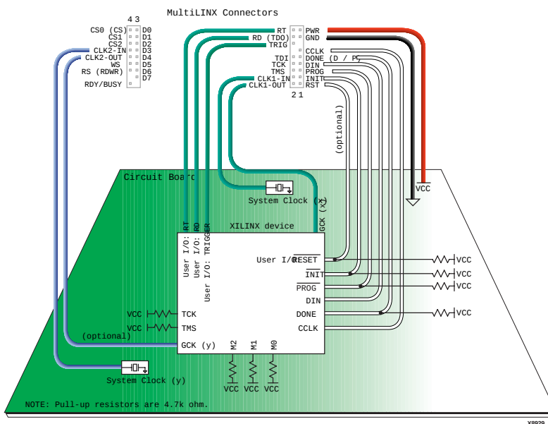
Figure 2-15 Slave Serial Mode (Spartan, XC5200, XC4000)
