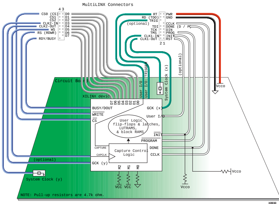
Figure 2-16 SelectMAP Mode (Virtex)
