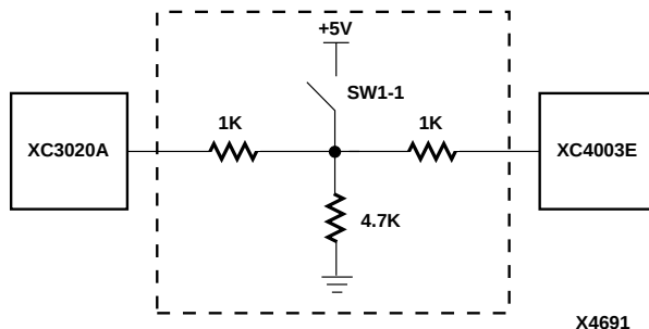
Figure 3-8 Configuration Switch SW1
