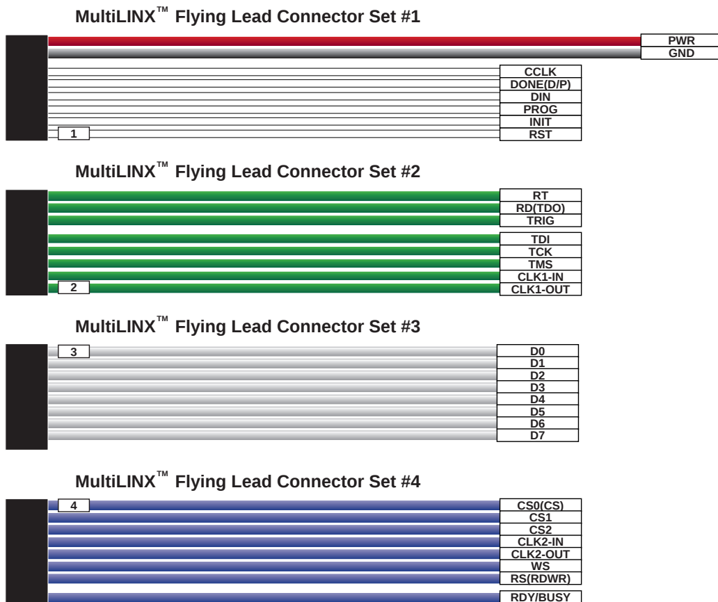
Figure 2-1 MultiLINX Flying Wires
