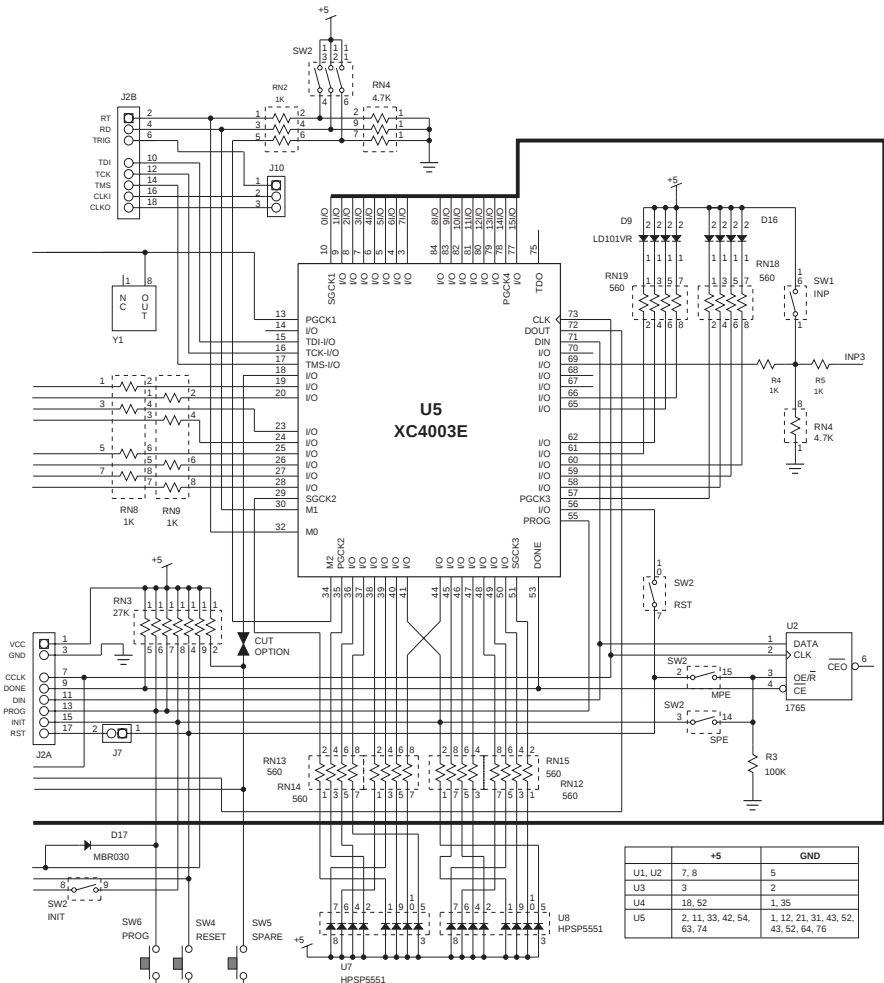
Figure 3-6 XC4003E Schematic
