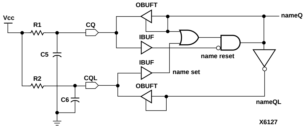
Figure 3-9 Relaxation Oscillator Schematic
