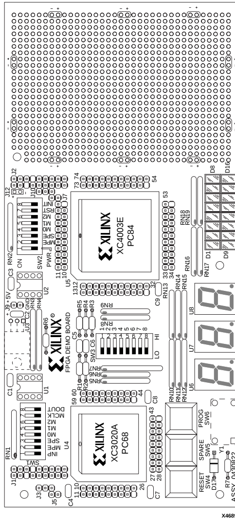
Figure 3-2 FPGA Demonstration Board
