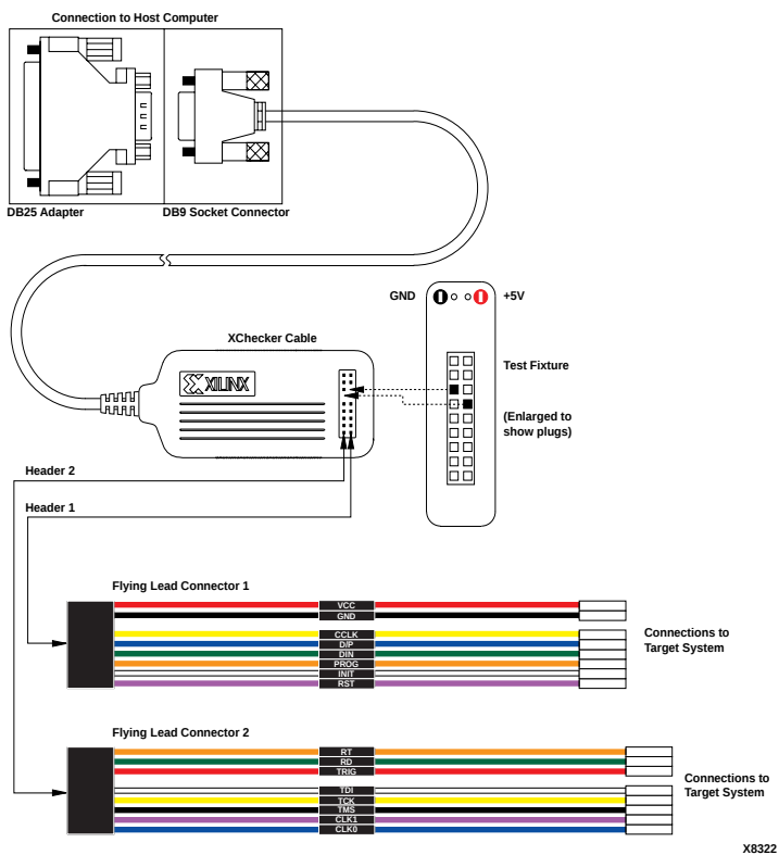
Figure 1-9 XChecker Cable and Flying Leads
