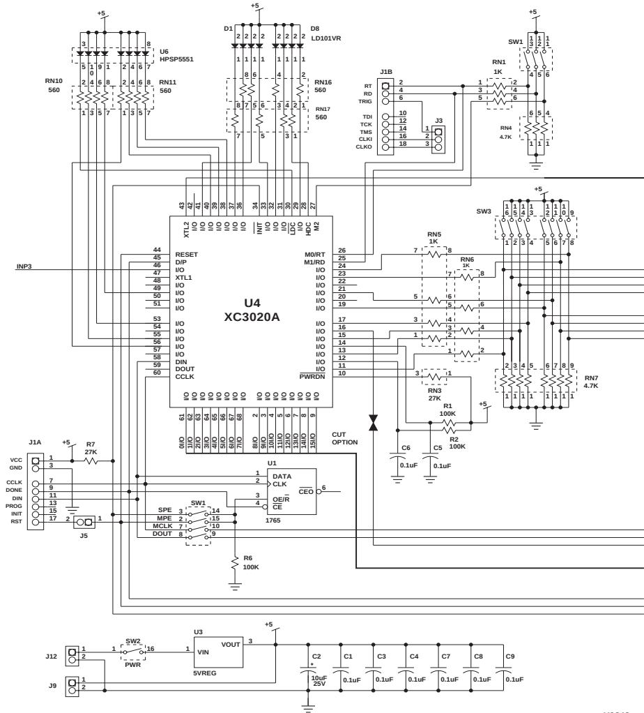
Figure 3-7 XC3020A Schematic
