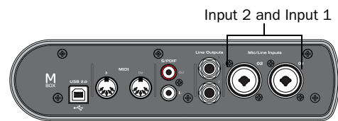
Inputs on rear panel of Mbox
