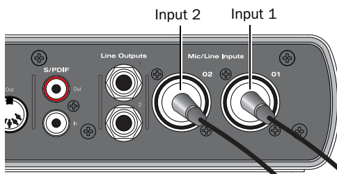
Mbox connections for line-level stereo input source
