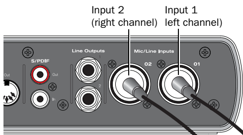
Mbox connections for line-level stereo input source
