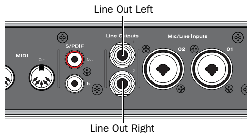
Stereo output from the Mbox (back panel)
