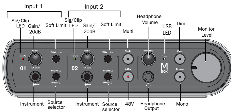
Figure 1. Mbox front panel
