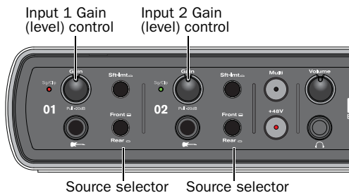
Source selector and Gain control for Inputs 1 and 2
