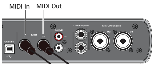
MIDI connections to Mbox
