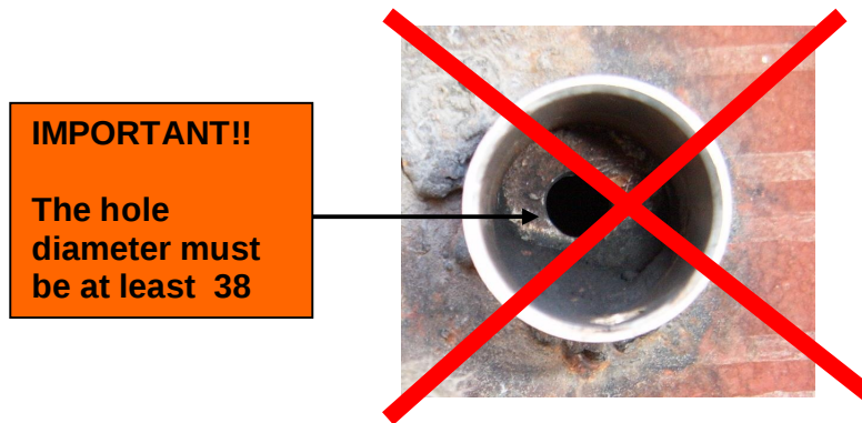
Figure 3b. Wrong socket installation, THE DIAMETER OF THE HOLE MUST BE MINIMUM 38 MM
