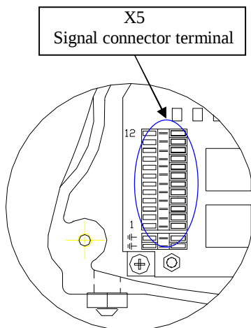
Figure 5a. Signal connector
