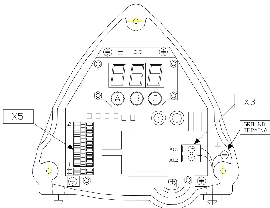
Figure 4. Wiring
