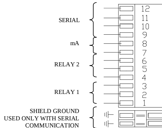
Figure 5b. Signal connector X5 wiring
