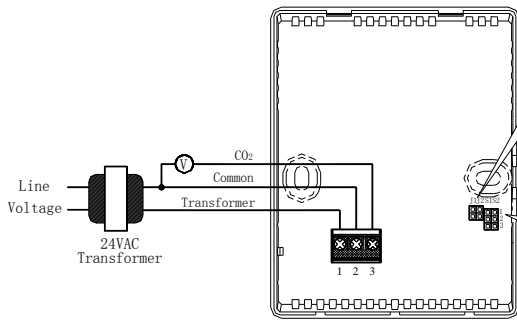
Figure.3 wiring diagram
