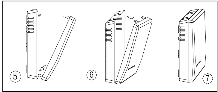
Figure.4 close it
