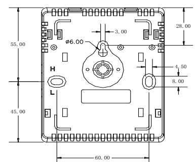
Figure.2 wall plate
