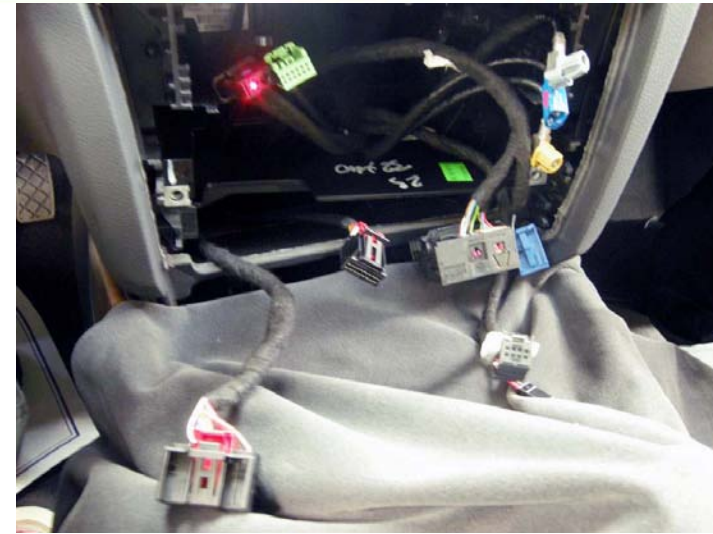
6. After disconnection.
