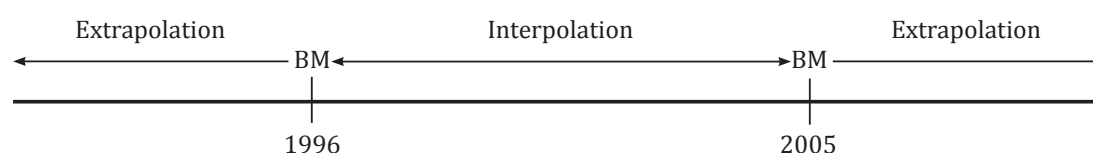
Figure 3, Schematic illustration of a hypothetical PPP computation
