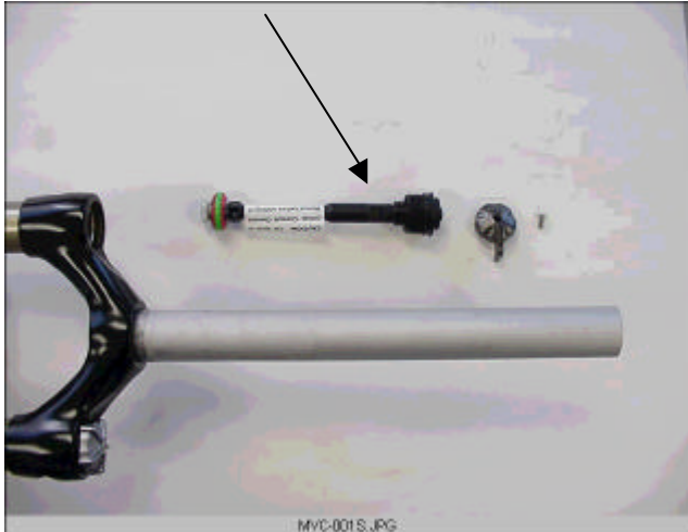
Compression Damping Assembly with Knob
