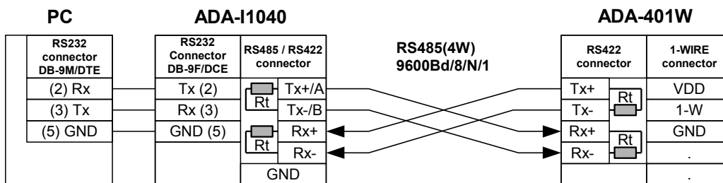
Fig. 3. 4-wire connection of ADA-401W to PC by the use of RS232 to RS485/RS422 converter ADA-I1040
