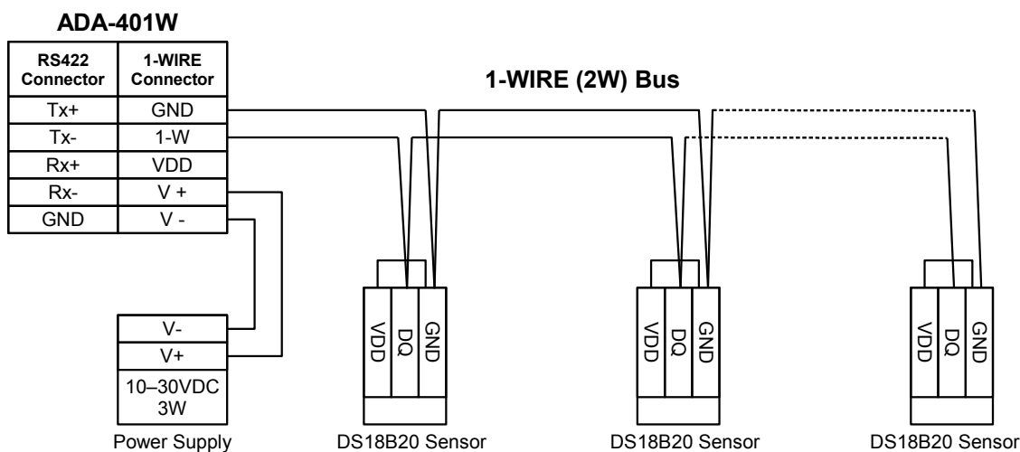
Fig. 6. Sensor connection to ADA-401W converter by 2-wire 1-WIRE Bus
