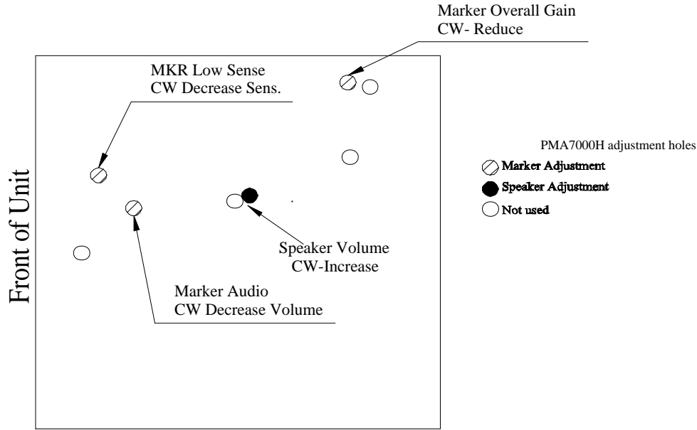
Figure 2-3- PMA7000H Adjustments
