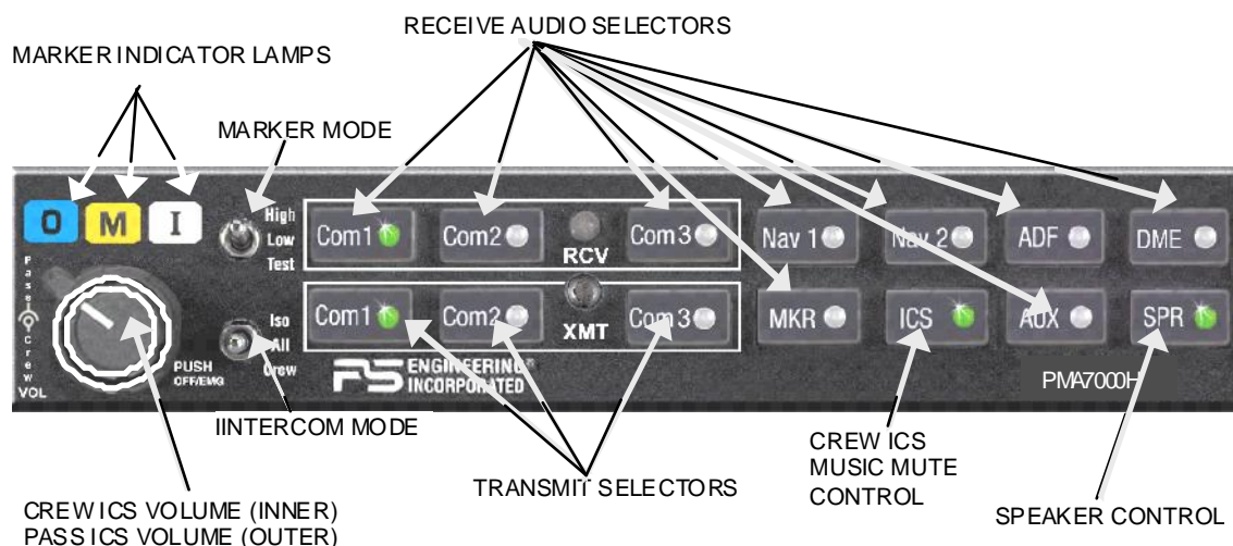
Figure 3-1 PMA7000H controls
