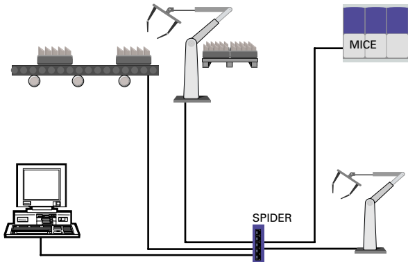
Fig. 4: Configuration with SPIDER 5TX: Connection of up to 8 data terminal equipments or further segments via TP
