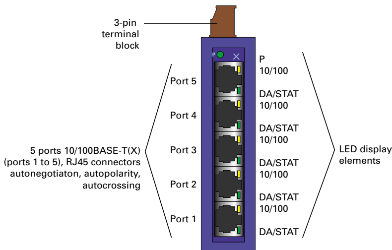
Fig. 1: Overview interfaces, display elements and controls
