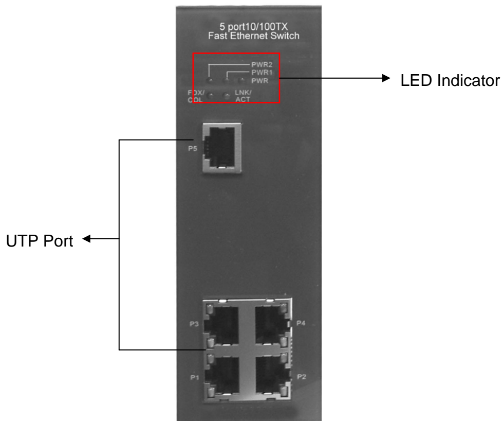
Figure A. Front Panel of the 5-port 10/100BaseTX Industrial Switch
