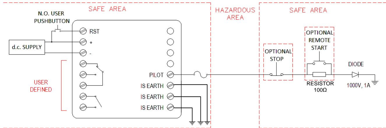
Figure 2: ECD Typical Electrical Application
