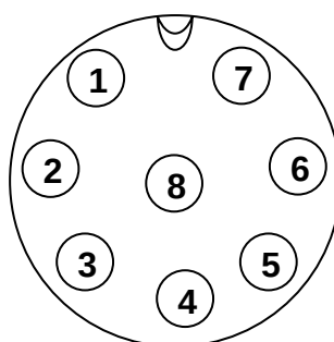
CONNECTOR BACK (SOLDER) END VIEW
