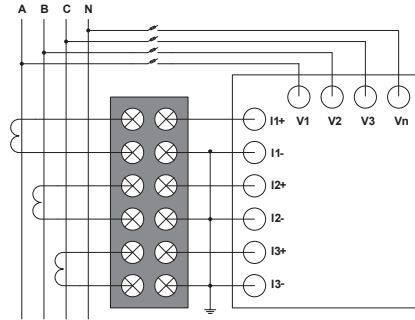
Diagram 5-6: Three-phase four-wire, Y-connection, 3 CT, No PT
