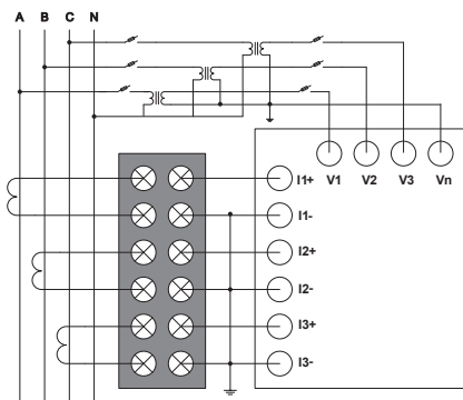
Diagram 5-7: Three-phase four-wire, Y-connection, 3 CT, 3 PT
