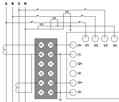
Diagram 5-8: Three-phase four-wire, Y-connection, 2 CT, 3 PT
