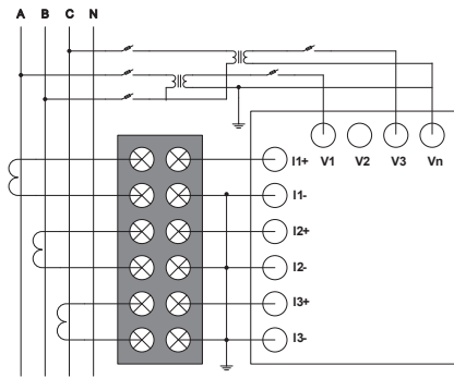
Diagram 5-5: Three-phase three-wire, \Delta Delta-connection, 3 CT, 2 PT
