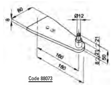
FRONT FIXING LONGER BRACKET TO SUIT 400 mm RAM
