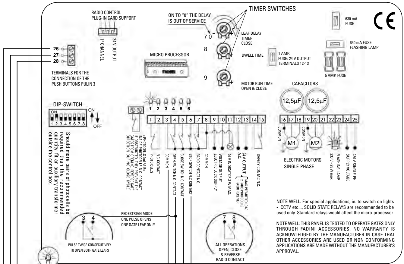
Drwg. No. 1643 P.C. BOARD
