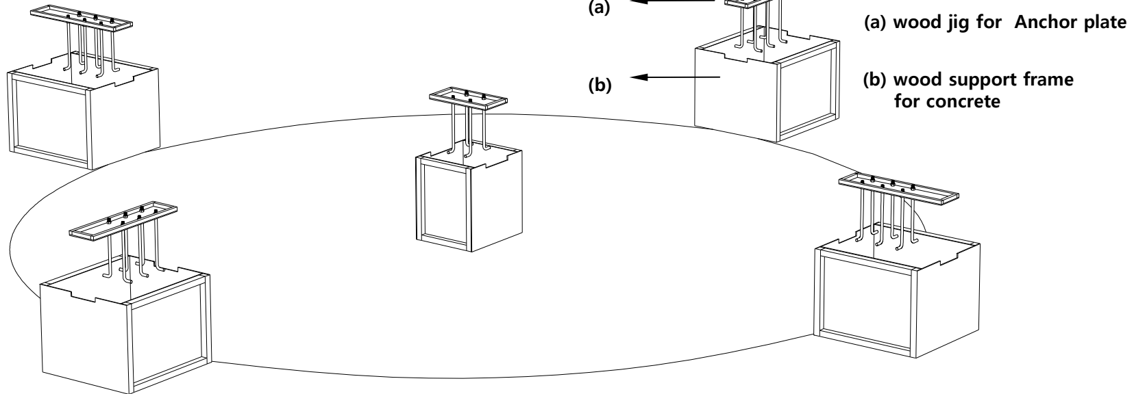
Figure-6: Wood support frame
