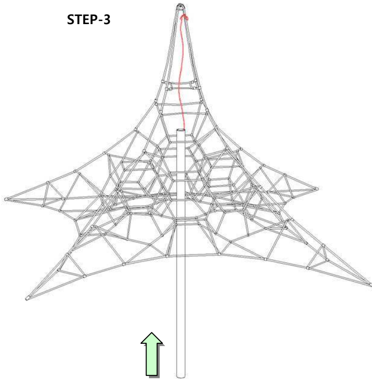
Figure-13: Insert Post into the Center of Net.
