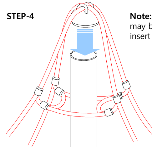
Figure-15: Post cap assembly.
