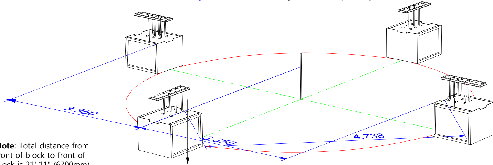
Figure-5: Concrete footing and Anchor plate layout
