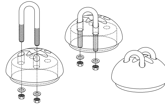
Figure-14: U-bolt assembly.
