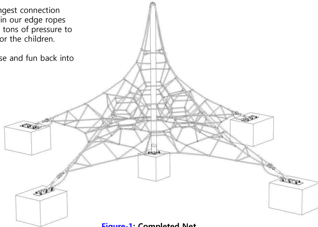
Figure-1: Completed Net
