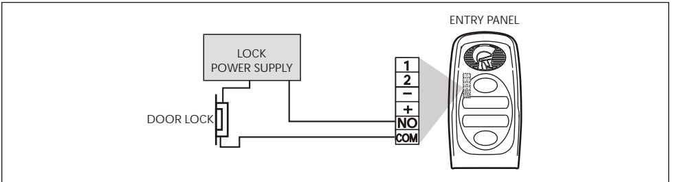
Fig 4 Door Lock Drive
