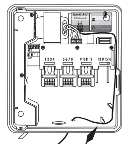
Communication cable routing guides.
