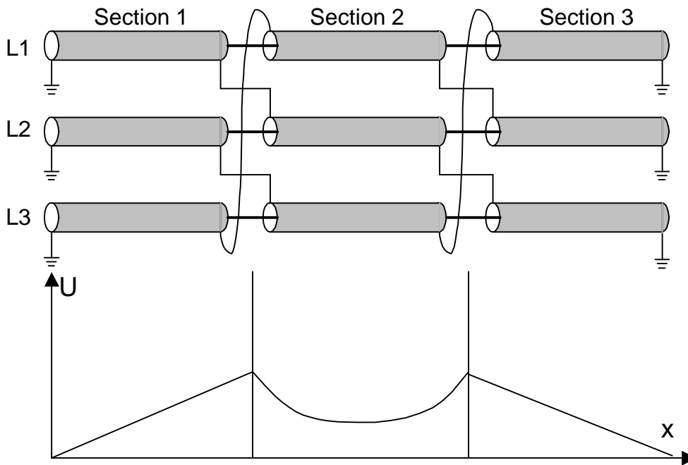
Induced voltage distribution at cross-bonding
