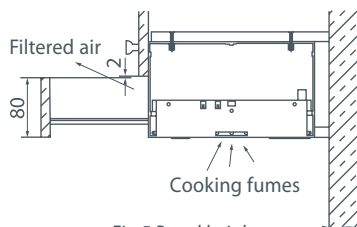
Fig.5 Panel heights
