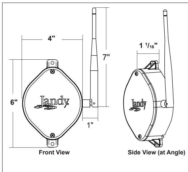
Figure 2. J-Box Transceiver Dimensions
