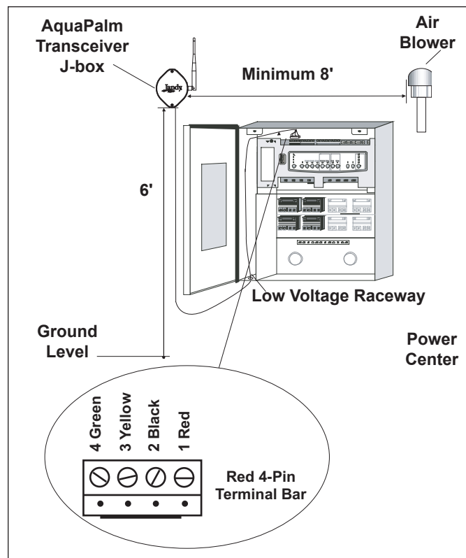
Figure 4. Outdoor Transceiver J-box Installation
