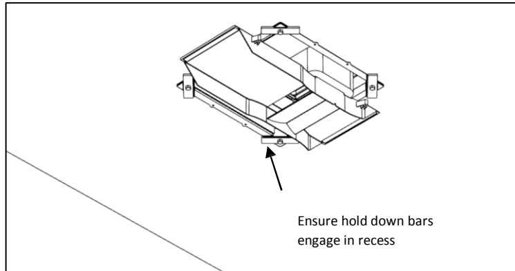
Fig 12: Engage the four M8 bolts, taking care to ensure the hold down bars slot into their recesses
