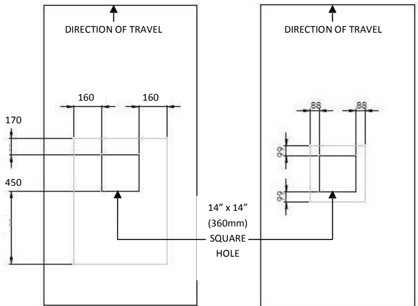
Fig 2: The foot print of the rooftop unit, and the plenum, measured from the 360 mm square hole
