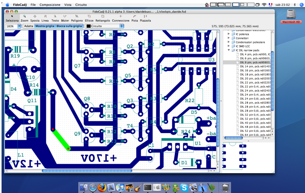
Figure 2.1.: A typical FidoCadJ session running on MacOSX Tiger. Appendix A describes the peculiarities of the version specific for Macintosh.
