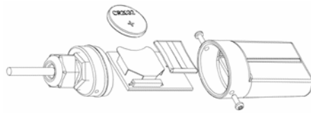
Figure 4: Battery Replacement
