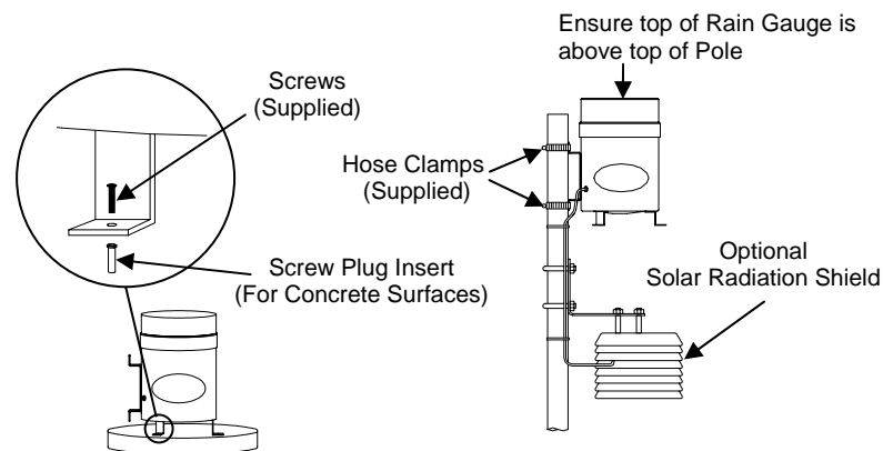
Figure 5: Surface Mounting
