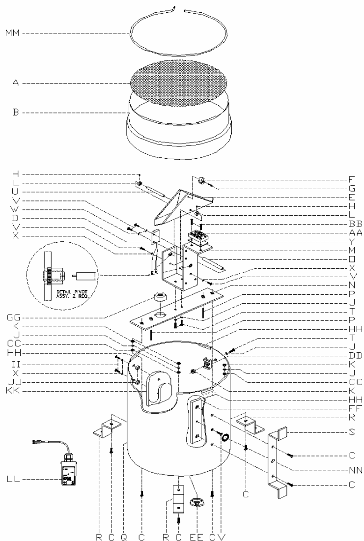
Figure 7: Rain Gauge Assembly
