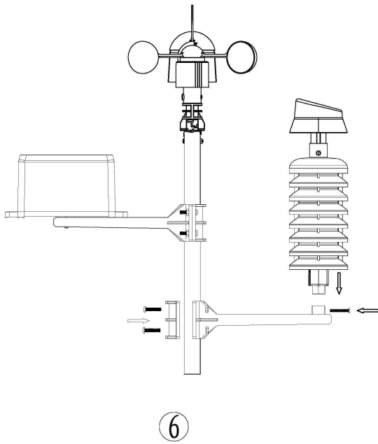
⑥ Mounting the thermo-hygro sensor same as rain sensor
