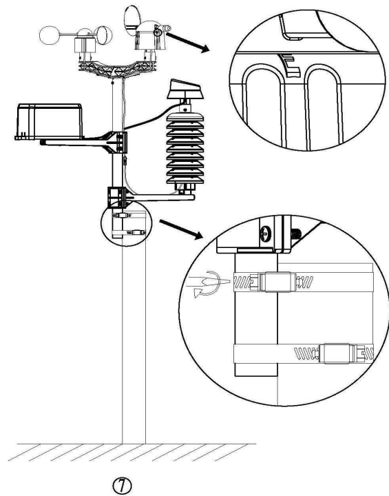
⑦ Fix the whole set to a pole with the two adjustable hoops.
