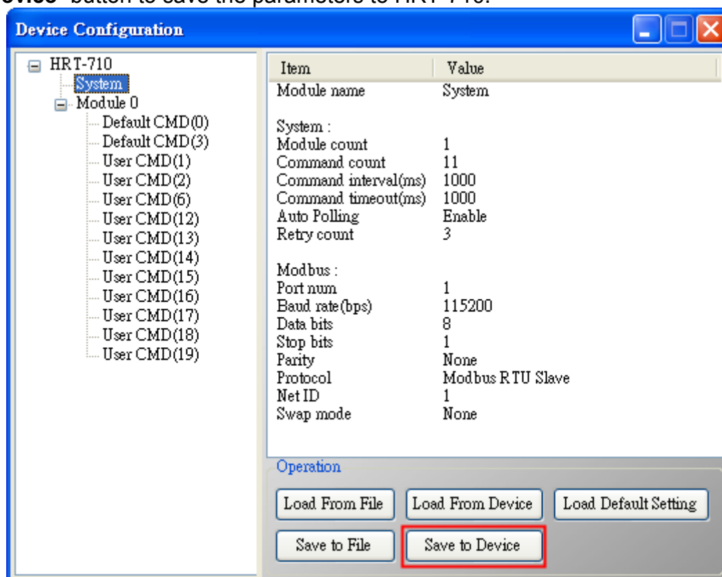
Figure 9-2 Setting for the RS-485 Station No. of HRT-710
