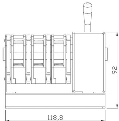
BTS-3P Drawing
