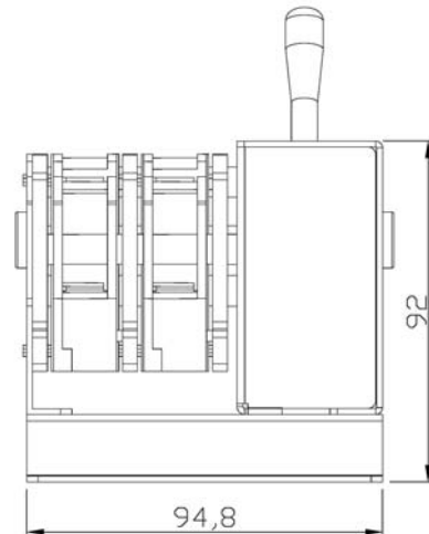
BTS-2P Drawing
